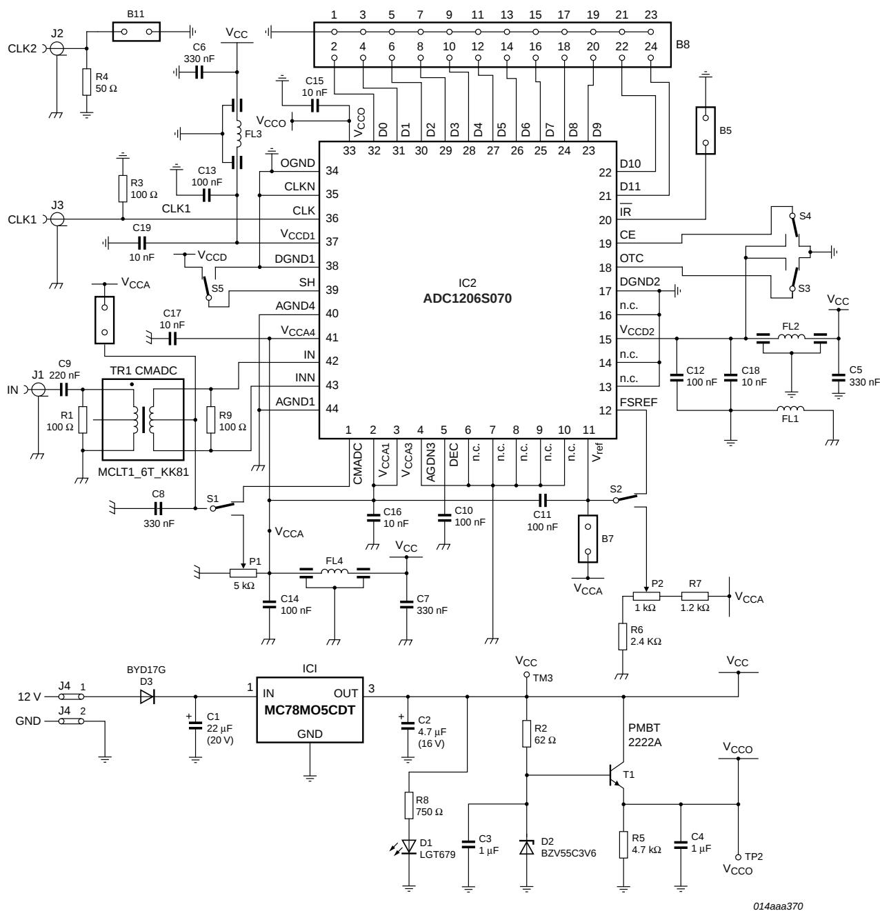
Fig 20. Demonstration board schematic.
