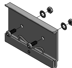
EXPLODED DINCLIP W/ HARDWARE
