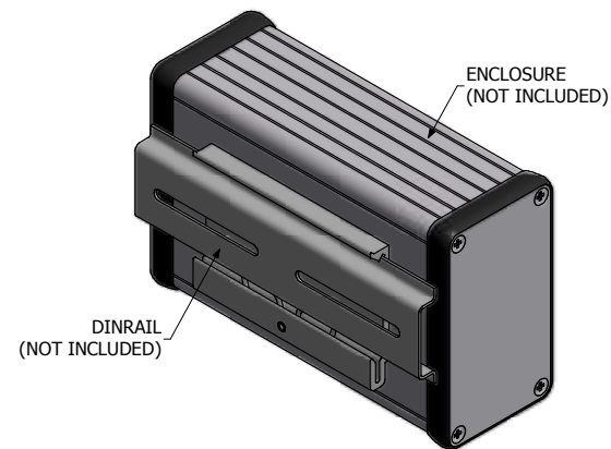
TYPICAL ASSEMBLY
