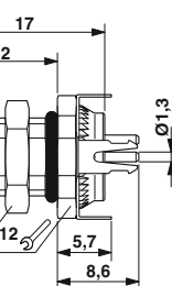
M8 flush-type plug, straight,
