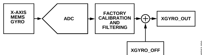
Figure 20. User Calibration, XGYRO_OFF Example
