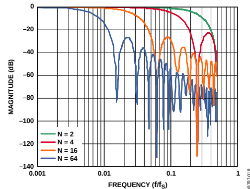
Figure 18. Bartlett Window, FIR Filter Frequency Response (Phase Delay = (2N_B - 1)/2 Samples)
