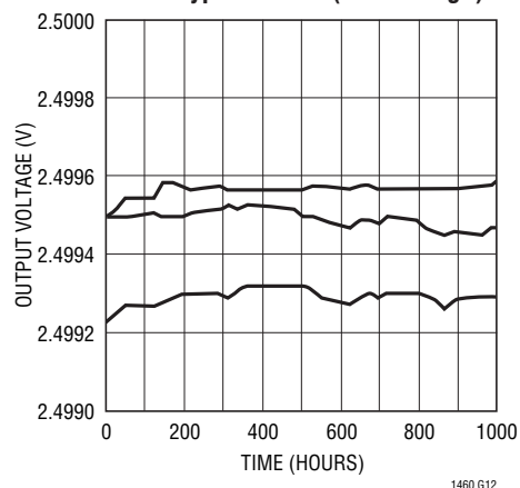
2.5V Long-Term Drift Three Typical Parts (S8 Package)
