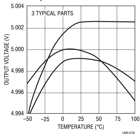
5V Output Voltage Temperature Drift
