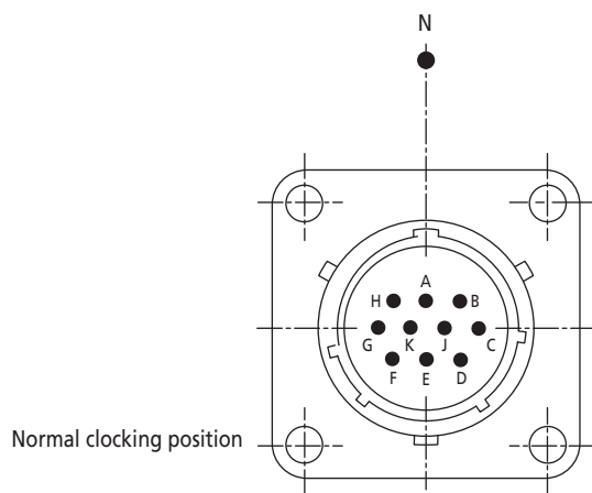
Exemple of insert angular displacement, pin front face view
