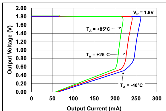
FIGURE 2-26: Output Voltage vs. Output Current.
