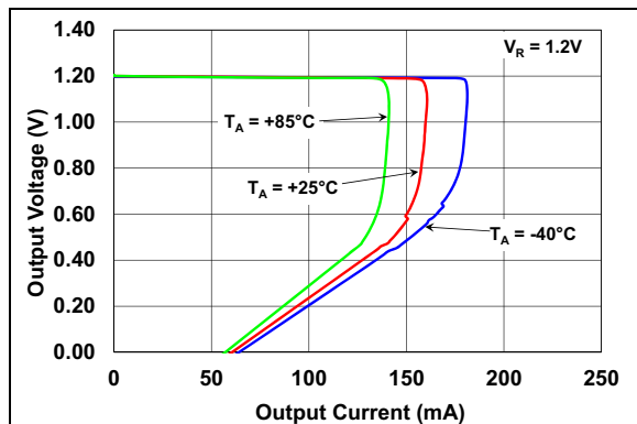
FIGURE 2-25: Output Voltage vs. Output Current.
