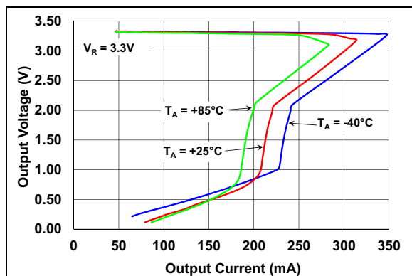
FIGURE 2-27: Output Voltage vs. Output Current.
