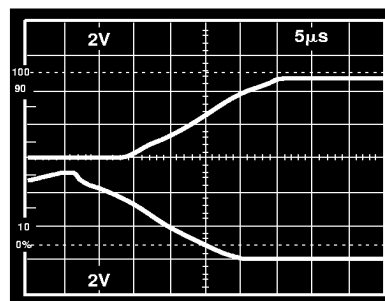
Figure 11. Precision Comparator
