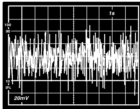
Figure 42. Input Voltage Noise @ +5 V ( 20 \text{ nV/div} )
