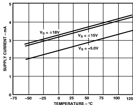
Figure 43. Supply Current vs. Temperature
