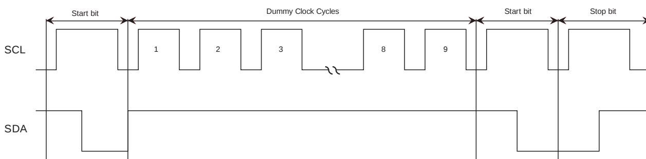
Figure 3. Software reset
