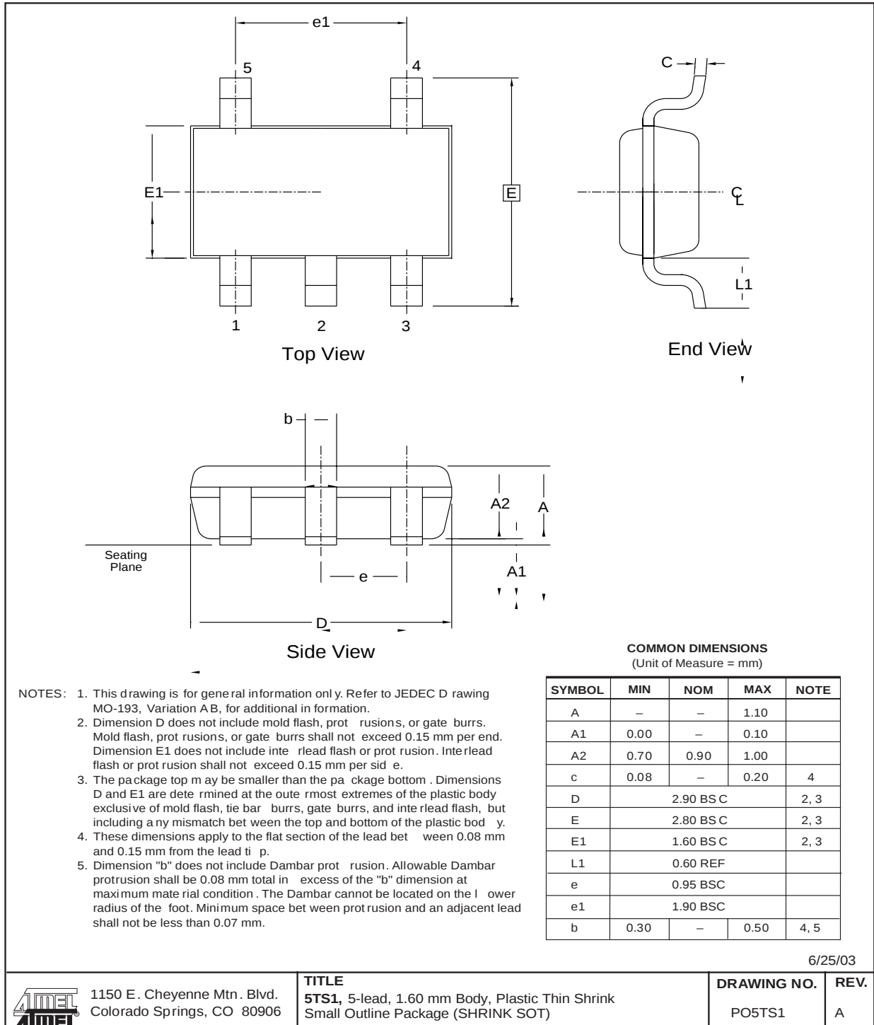
Figure 19. 5TS1 – SOT23
