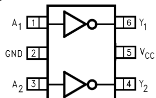
Figure 2. SC70 (Top View)
