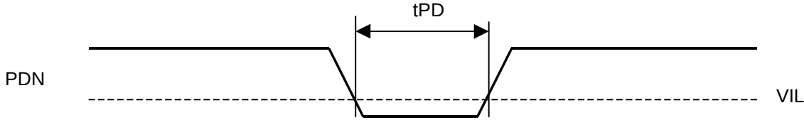
Power-down Timing
