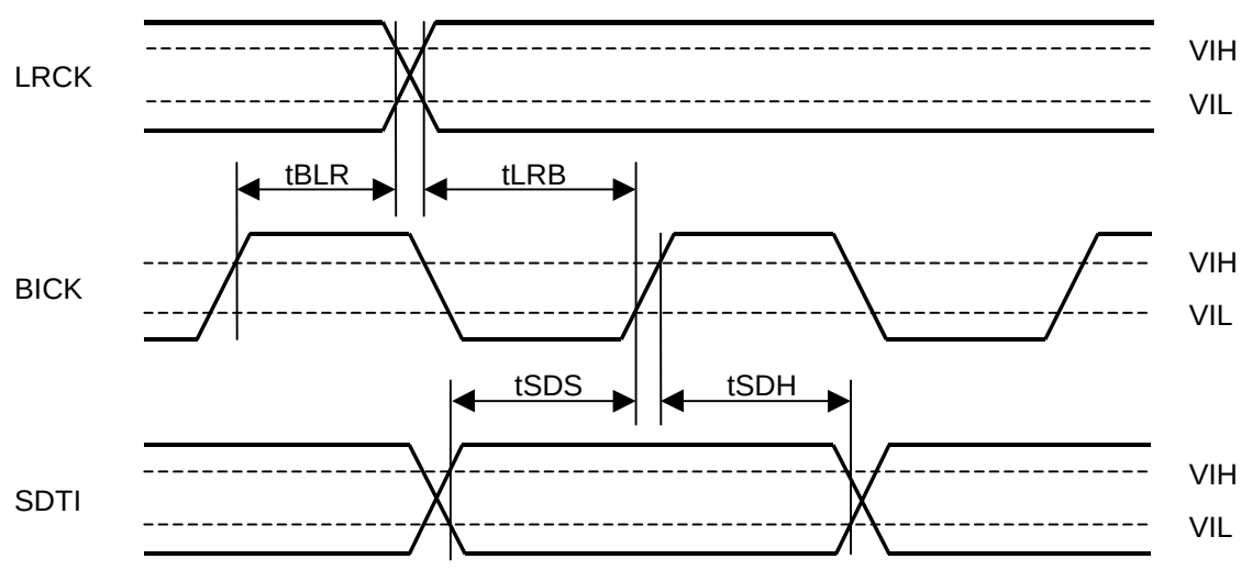
Serial Interface Timing
