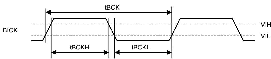
Clock Timing
