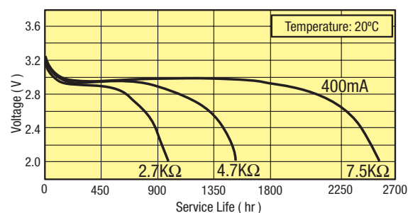
TYPICAL CR2477 DISCHARGE CHARACTERISTICS AT VARIED RATES
