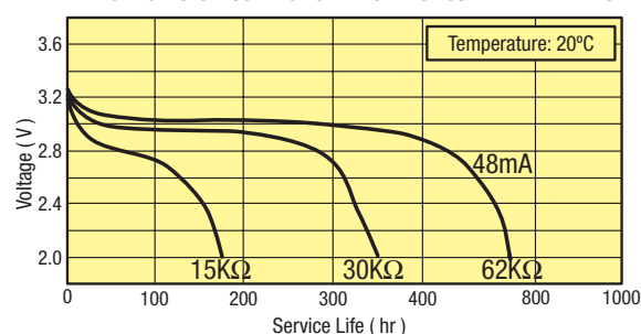
TYPICAL CR2032 DISCHARGE CHARACTERISTICS AT VARIED RATES
