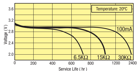
TYPICAL CR2477 DISCHARGE CHARACTERISTICS AT VARIED RATES
