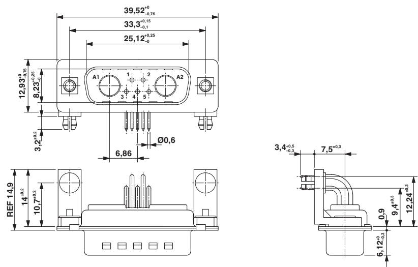
Dimensioned drawing
