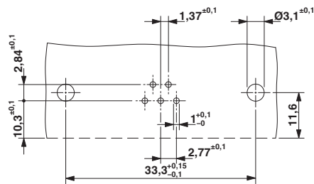
Drilling diagram
