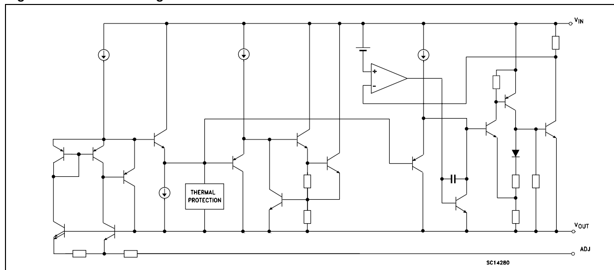
Figure 1: Schematic Diagram
