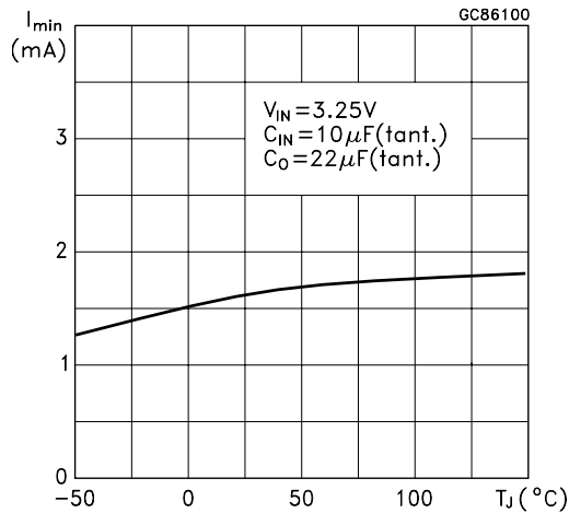
Figure 19: Stability
