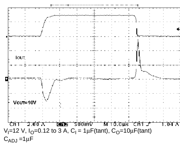
Figure 24: Load Transient
