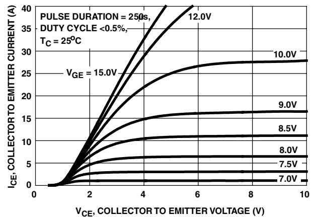
FIGURE 2. SATURATION CHARACTERISTICS
