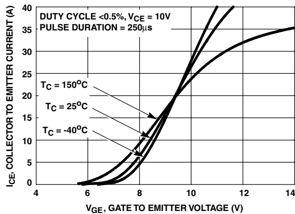
FIGURE 1. TRANSFER CHARACTERISTICS
