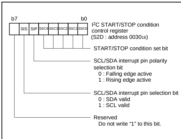
Fig. 38 Structure of I²C START/STOP condition control register
