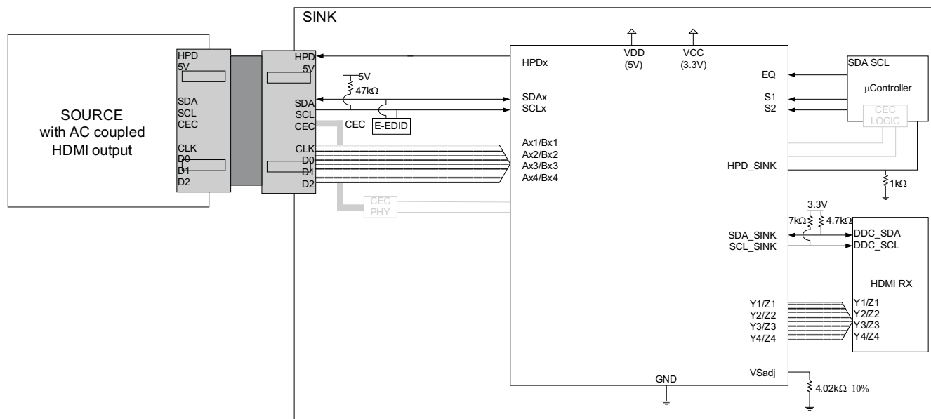
Figure 19. Two-Port HDMI Enabled DTV with TMD5251 – AC Coupled Source - CEC Commands Active
