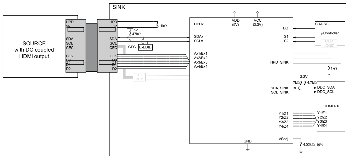
Figure 20. Two-Port HDMI Enabled DTV with TMD5251 – DC Coupled Source - CEC Commands Active
