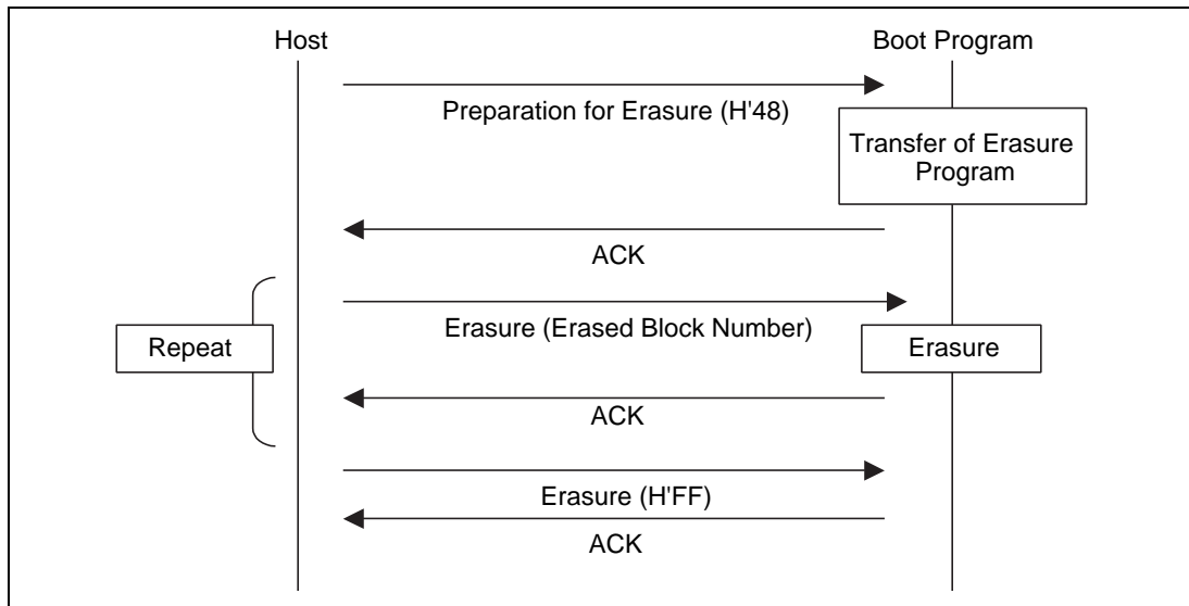
Figure 18.28 Erasure Sequence
