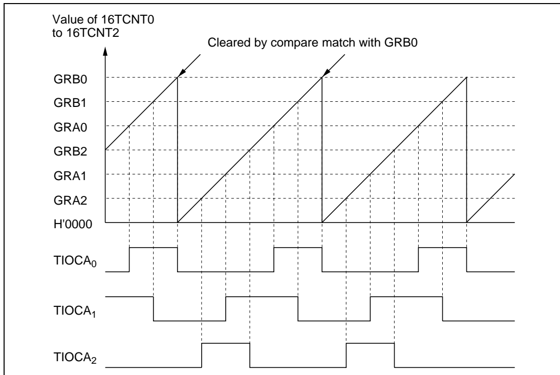
Figure 9.25 Synchronization (Example)
