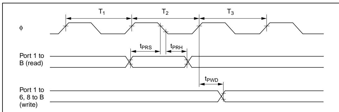
Figure 21.22 TPC and I/O Port Input/Output Timing
