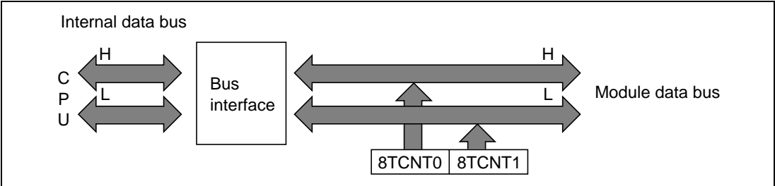
Figure 10.3 8TCNT Access Operation (CPU Reads 8TCNT, Word)
