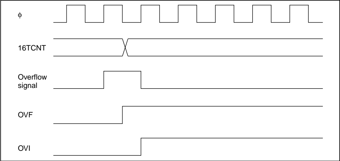
Figure 9.35 Timing of Setting of OVF
