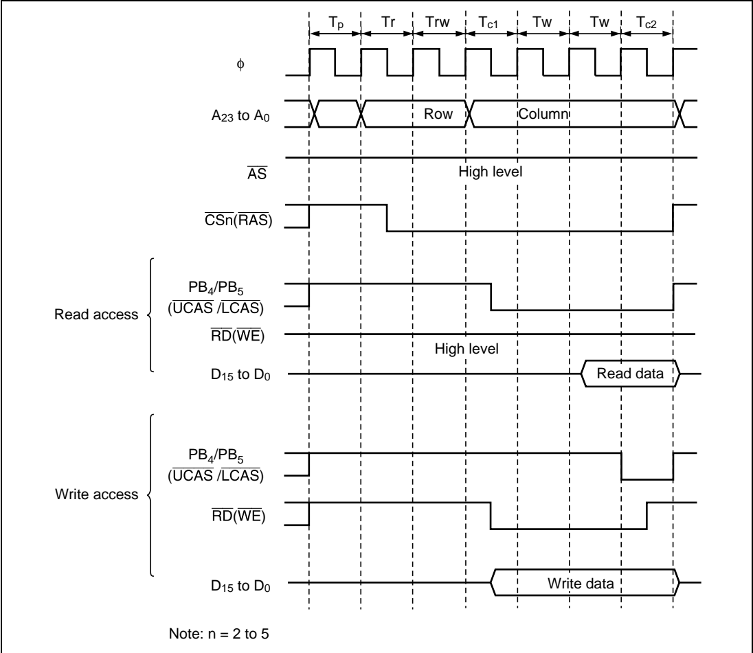
Figure 6.20 Example of Wait State Insertion Timing (CSEL = 0)
