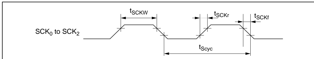
Figure 21.25 SCI Input Clock Timing
