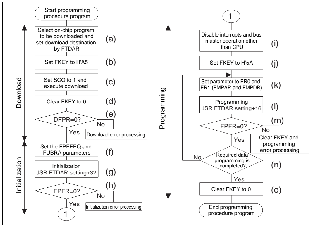
Figure 18.11 Programming Procedure
