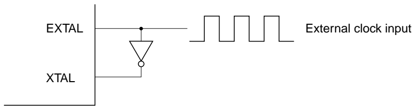
(a) Complementary clock input at XTAL pin
