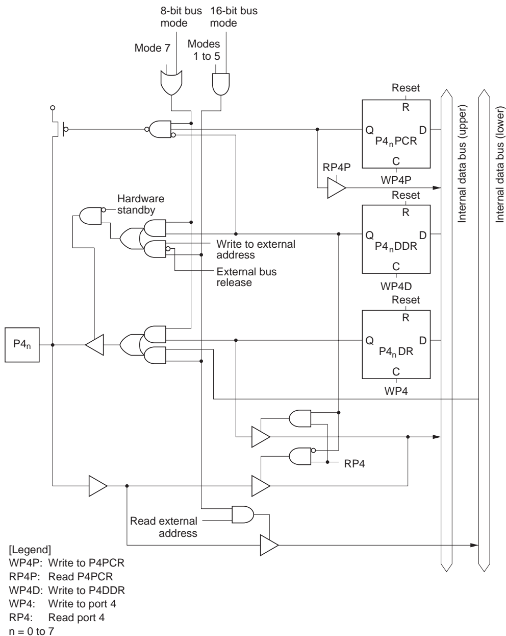
Figure C.4 Port 4 Block Diagram
