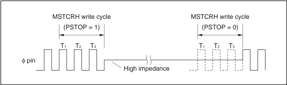
Figure 20.4 Starting and Stopping of System Clock Output
