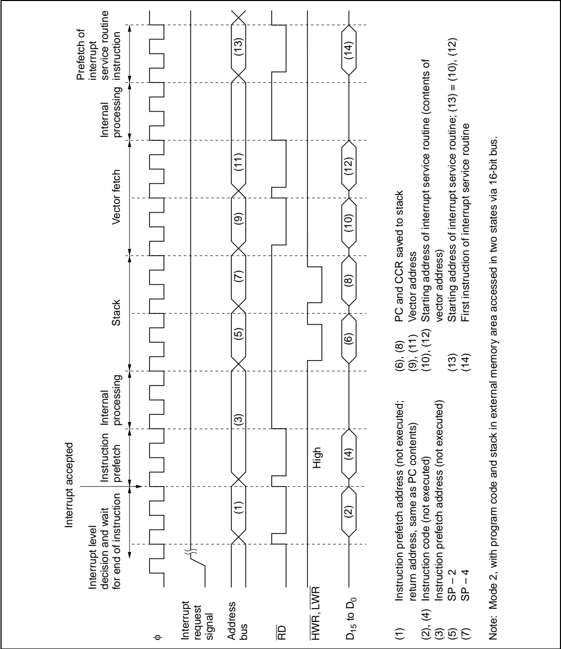
Figure 5.7 Interrupt Sequence
