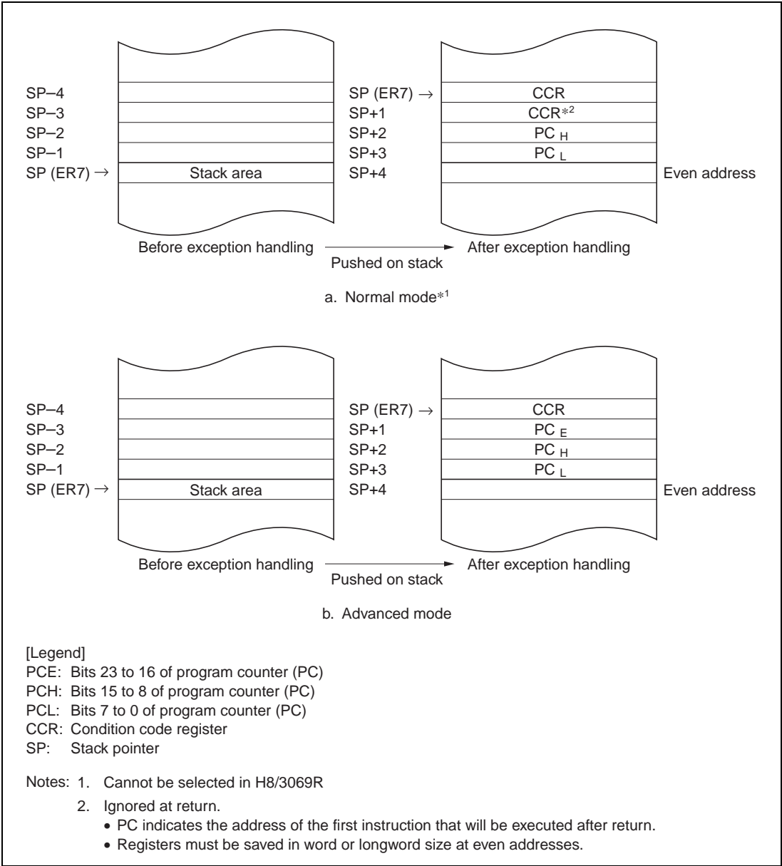
Figure 4.5 Stack after Completion of Exception Handling
