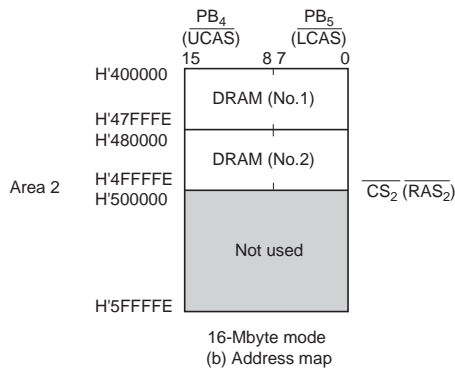
(b) Address map
