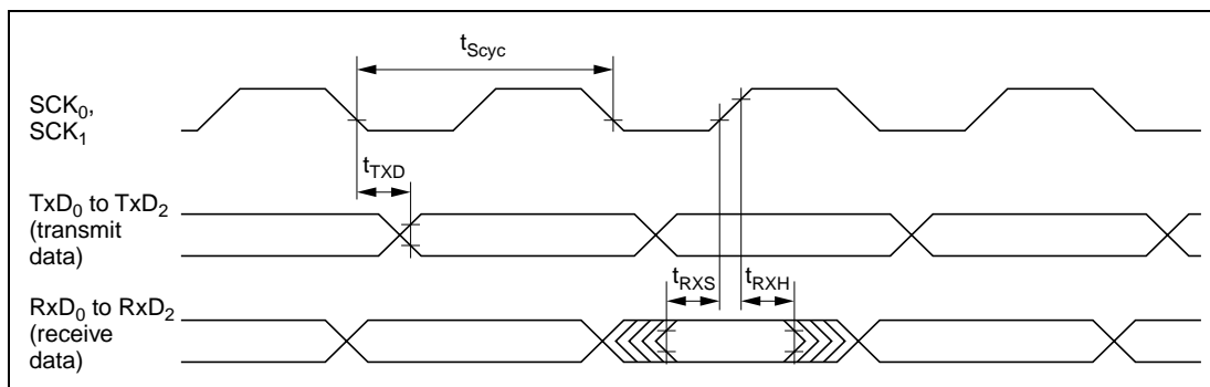
Figure 21.26 SCI Input/Output Timing in Synchronous Mode
