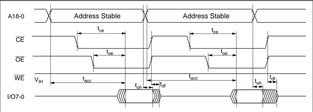
Figure 18.32 \overline{\text{CE}}/\overline{\text{OE}} Clock Read
