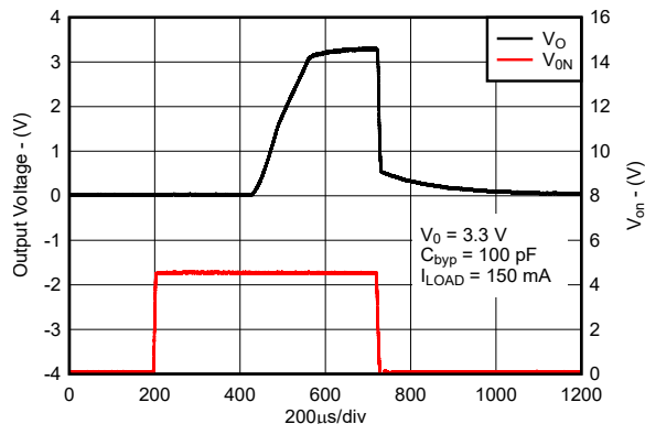
Figure 7-18. Turn-On Time for New Chip
