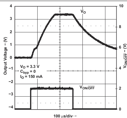
Figure 7-17. Turn-On Time for Legacy Chip
