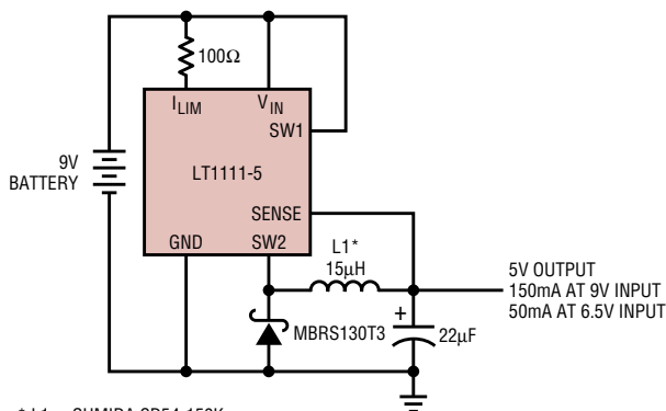
9V to 5V Step-Down Converter
