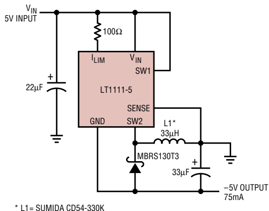
5V to -5V Converter
