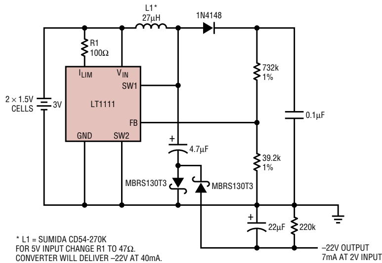
3V to -22V LCD Bias Generator
