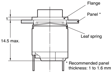
Panel Mounting Dimensions
