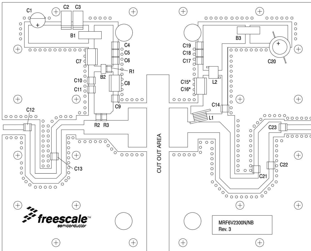
Figure 3. MRF6V2300NR1(NBR1) Test Circuit Component Layout — 220 MHz
