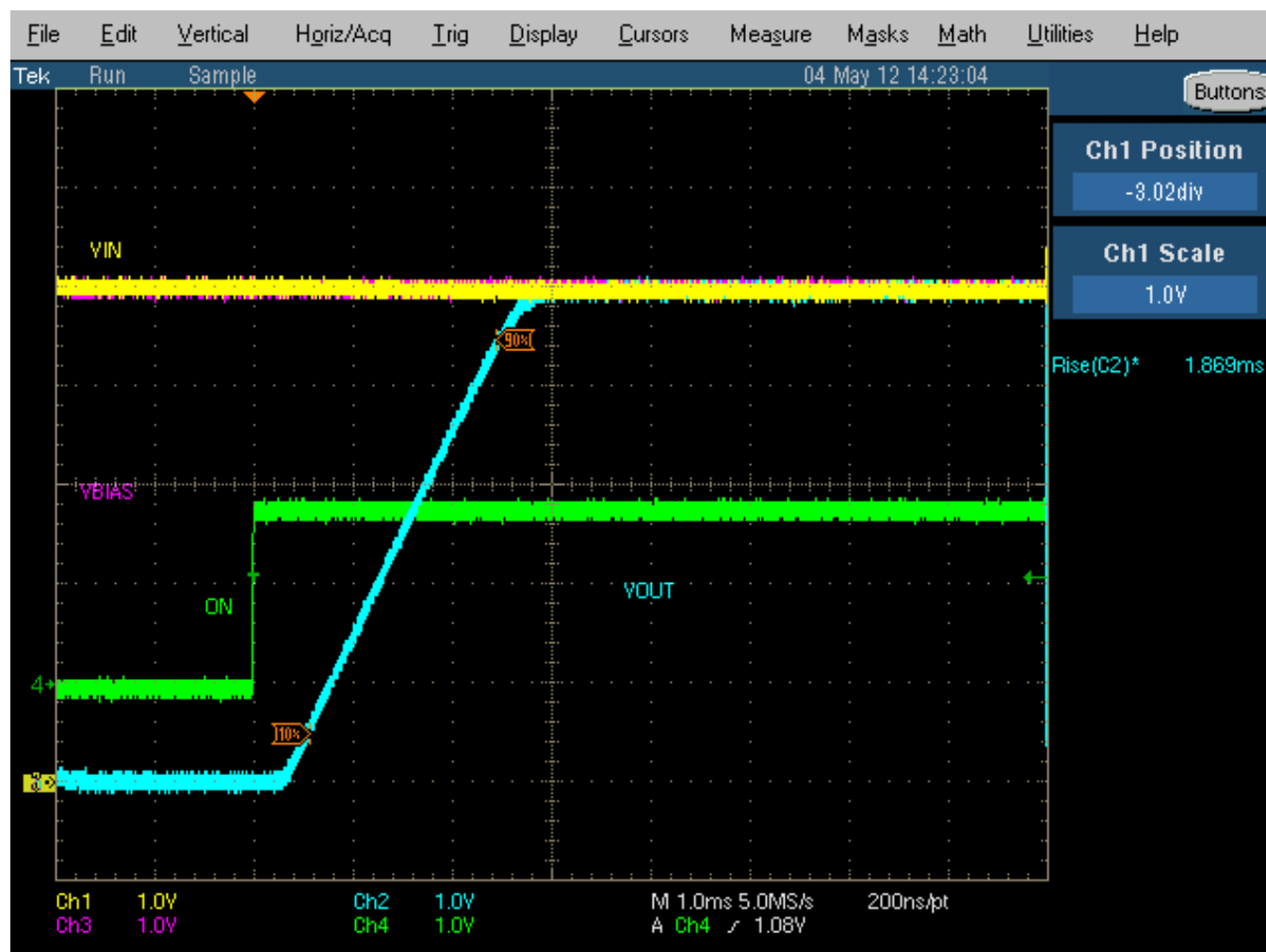
Figure 7. TPS22965EVM-023 Trise VIN = 5 V, ct = 1nF, and Load = 10 \Omega
