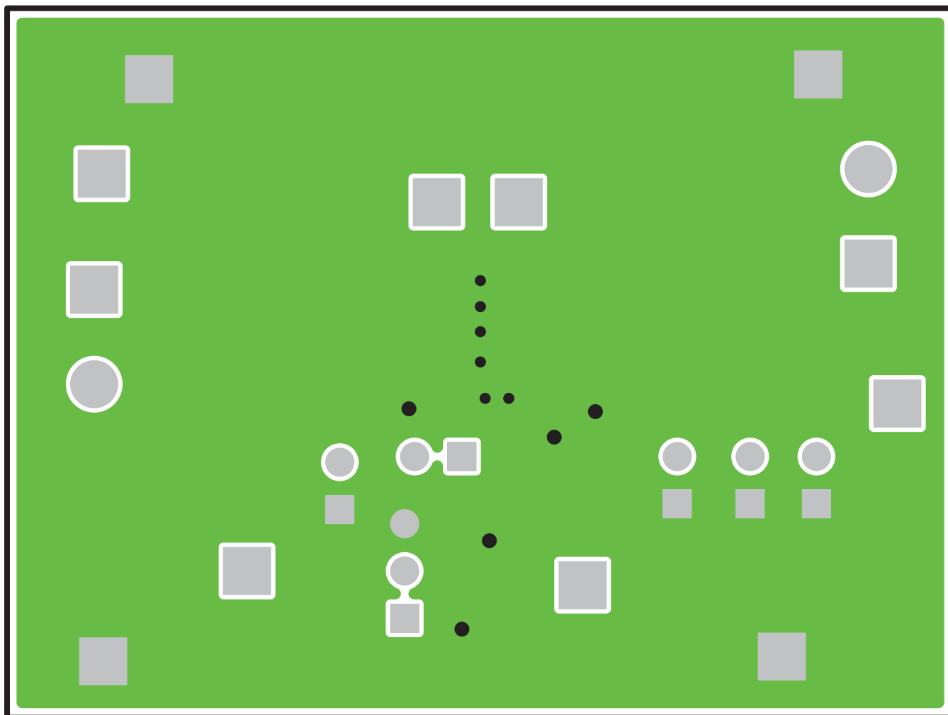
Figure 4. TPS22965EVM-023 Bottomside
