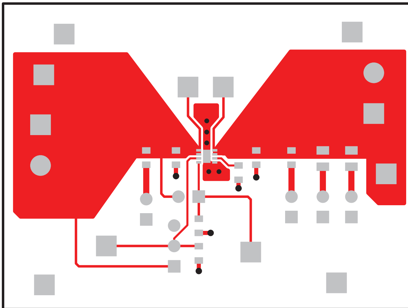
Figure 3. TPS22965EVM-023 Topside
