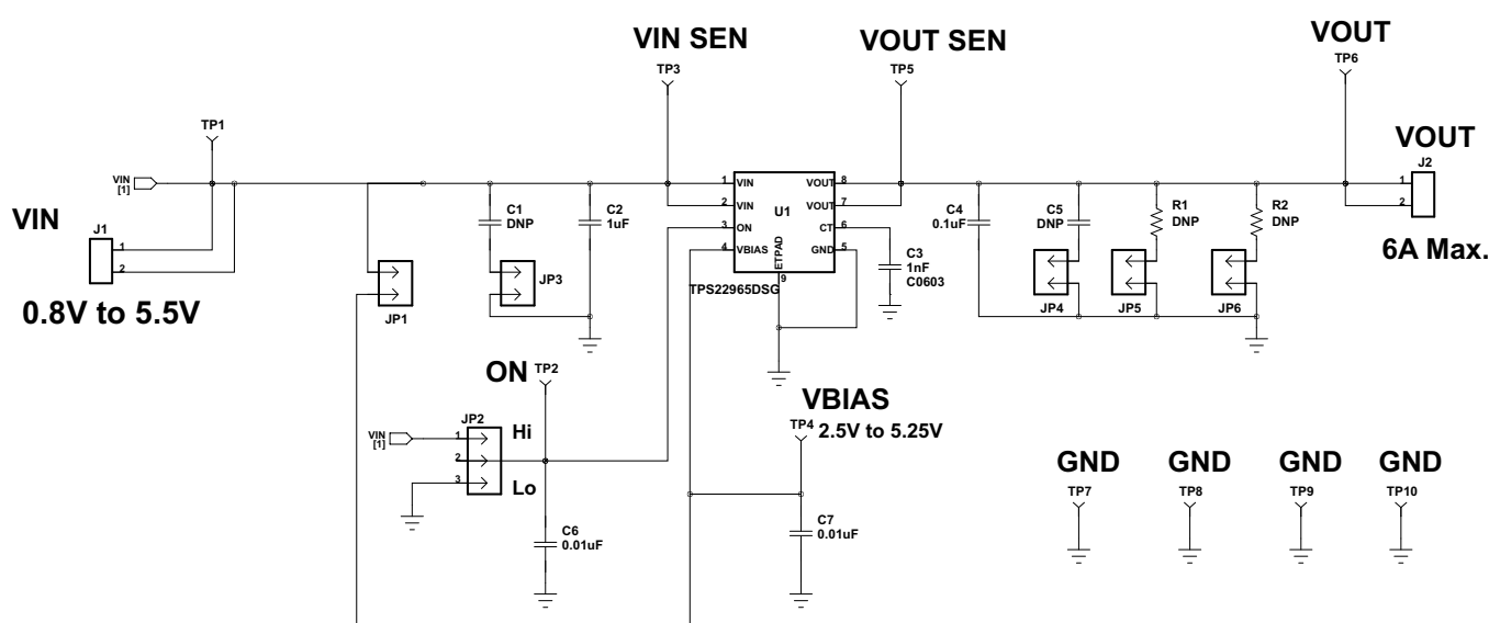
Figure 1. TPS22965EVM-023 Schematic
