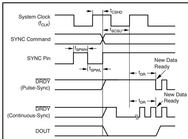
Figure 52. Pulse-Sync Timing, Continuous-Sync Timing with Single Sync
