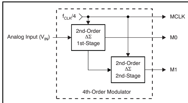
Figure 36. Fourth-Order Modulator
