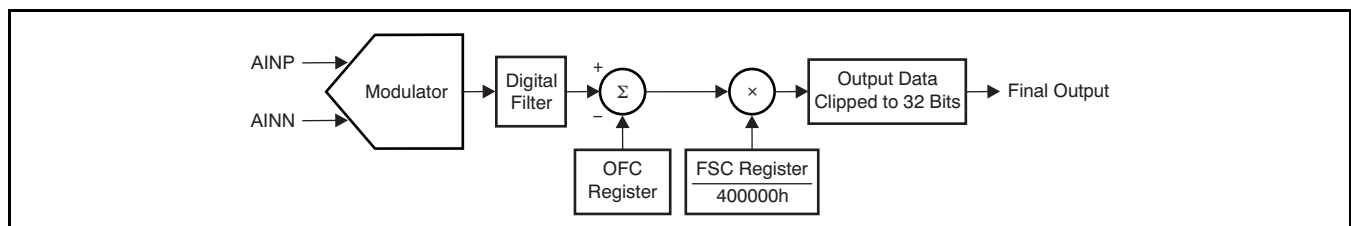
Figure 64. Calibration Block Diagram
