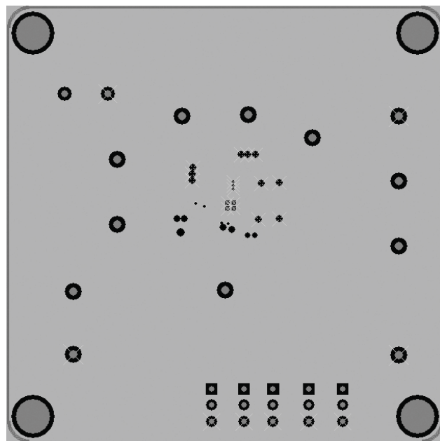
b: Internal Plane 1 (AGND)
