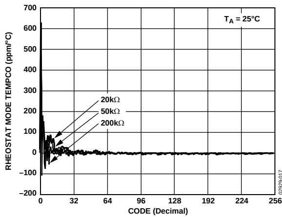
Figure 17. Rheostat Mode Tempco \Delta R_{\text{WB}}/\Delta T vs. Code, V_{\text{DD}}/V_{\text{SS}} = \pm 5\text{V}
