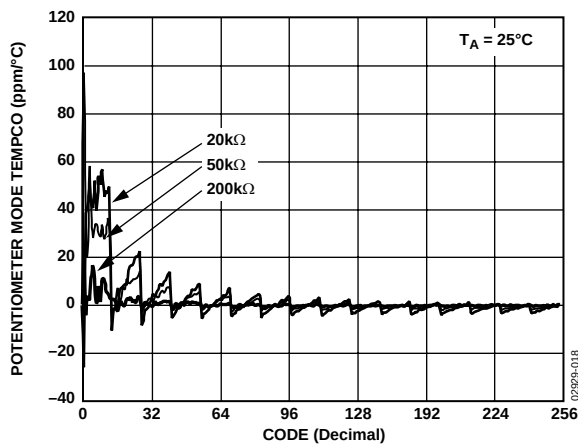
Figure 18. Potentiometer Mode Tempco \Delta V_{\text{WB}}/\Delta T vs. Code, V_{\text{DD}}/V_{\text{SS}} = \pm 5\text{V}
