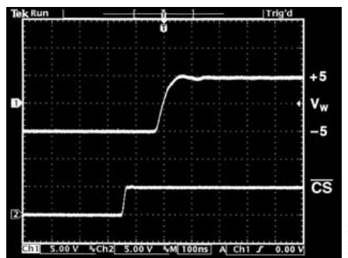
Figure 27. Large Signal Settling Time
