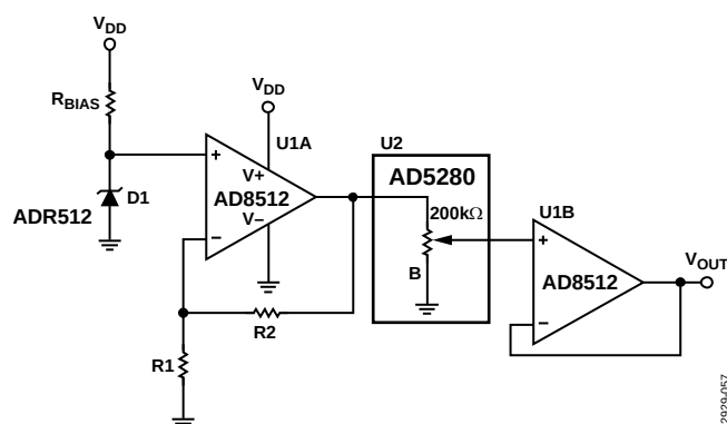
Figure 56. 8-BIT I 2 C DAC
