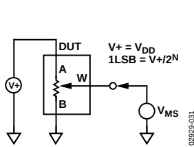
Figure 31. Potentiometer Divider Nonlinearity Error (INL, DNL)
