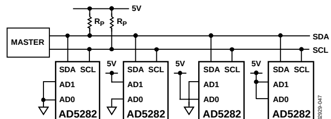
Figure 47. Multiple AD5282 Devices on One Bus
