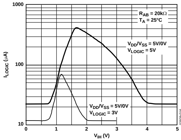
Figure 16. V_{\text{LOGIC}} Supply Current vs. Digital Input Voltage
