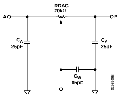
Figure 64. RDAC Circuit Simulation Model for RDAC = 20 k \Omega
