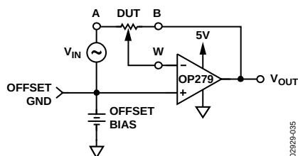
Figure 35. Inverting Gain
