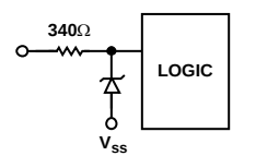
Figure 51. ESD Protection of Digital Pins
