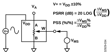
Figure 34. Power Supply Sensitivity (PSS, PSRR)
