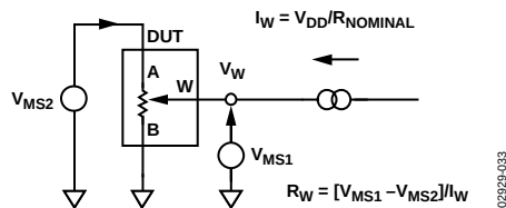
Figure 33. Wiper Resistance
