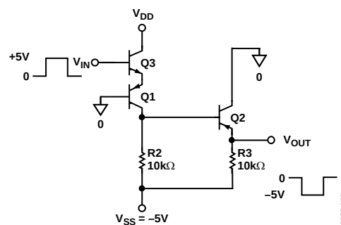
Figure 50. Level Shift for Bipolar Potential Operation
