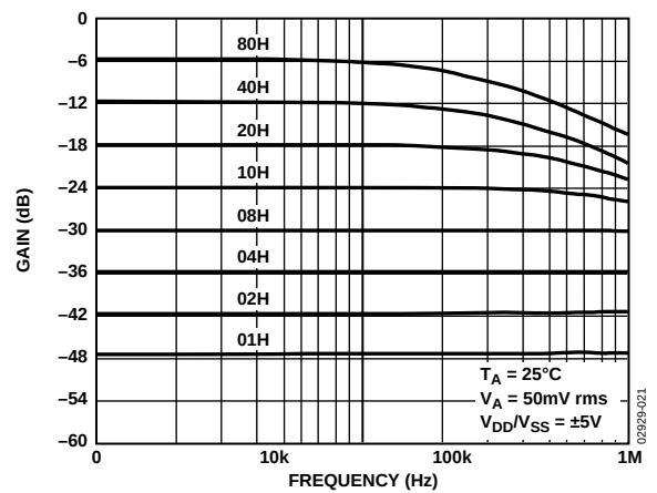
Figure 21. Gain vs. Frequency vs. Code, R_{\text{AB}} = 200\text{ k}\Omega
