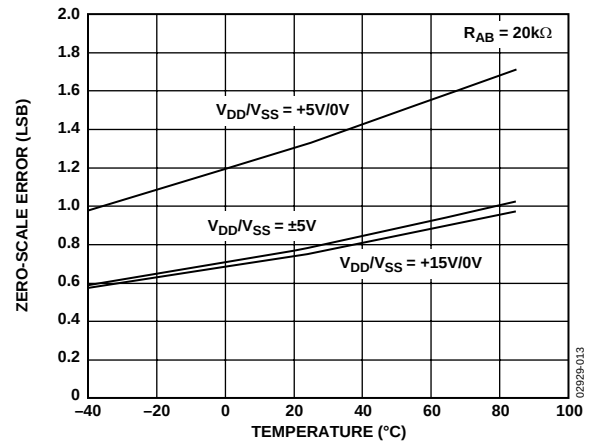
Figure 13. Zero-Scale Error
