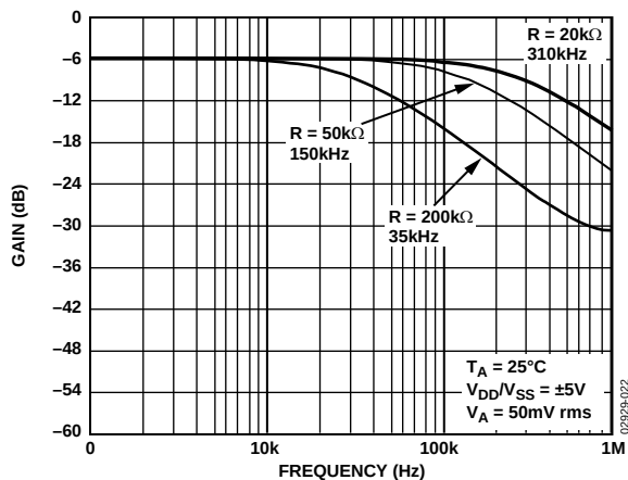
Figure 22. -3 dB Bandwidth
