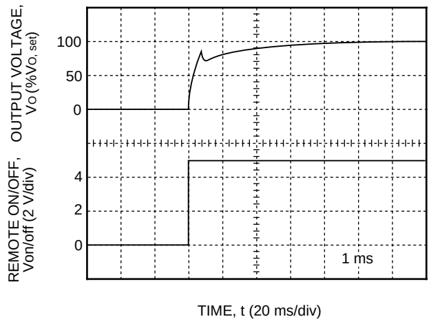
Figure 18. Typical A, B, C, D, F Output Voltage Start-Up when Signal Applied to Remote On/Off
