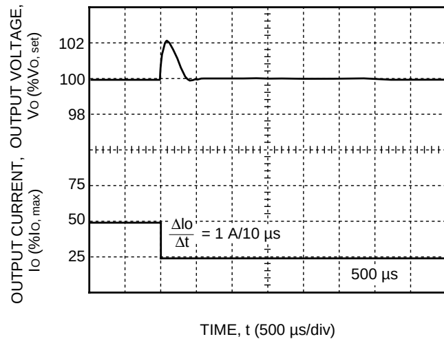
Figure 17. Typical A, B, C, D, F Output Voltage for a Step Load Change from 50% to 25%
