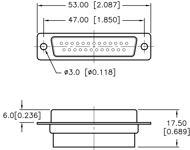
DB25(M)
