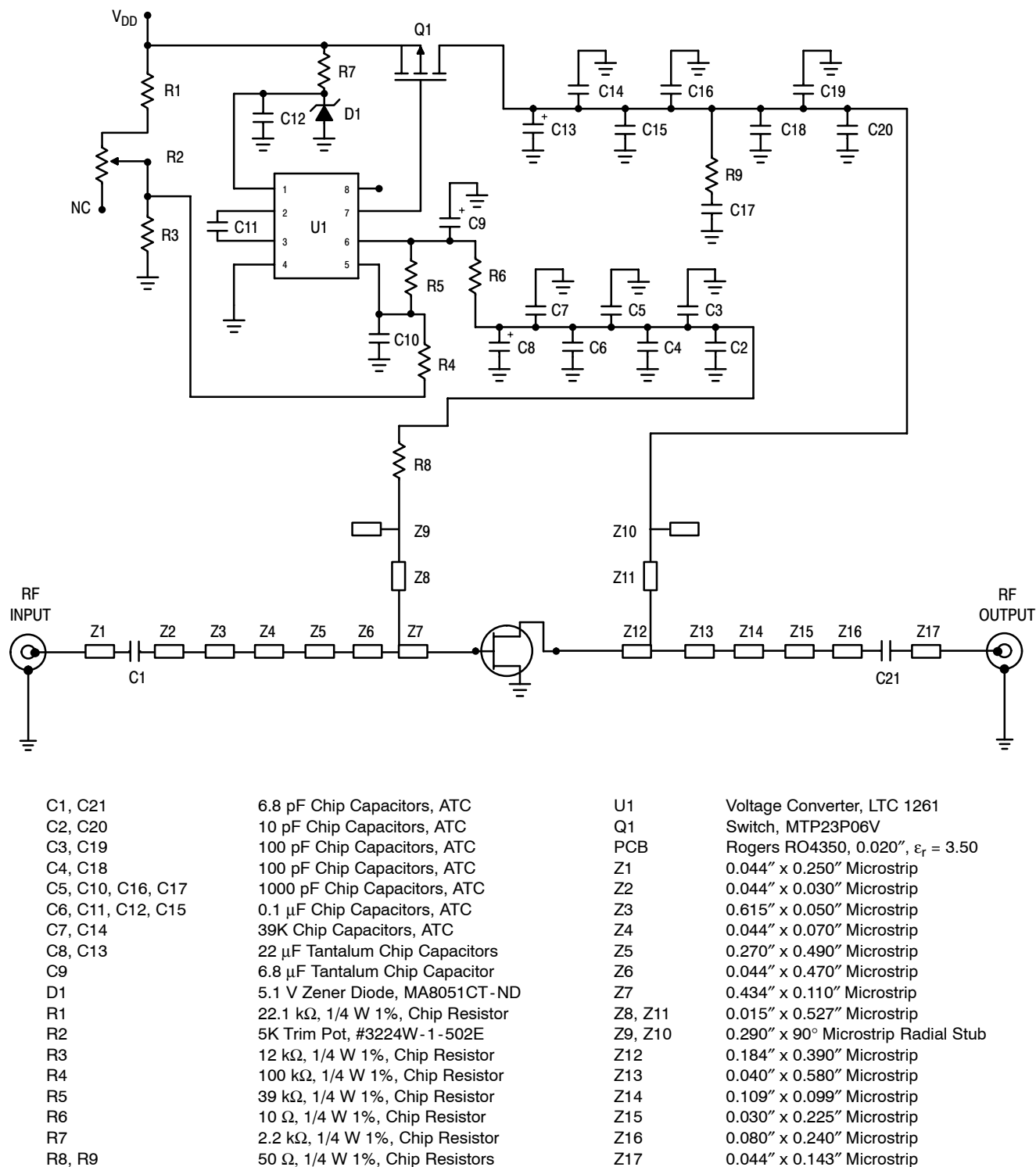
Figure 1. 3.4 - 3.6 GHz Single Supply Bias Sequencing Test Circuit Schematic
