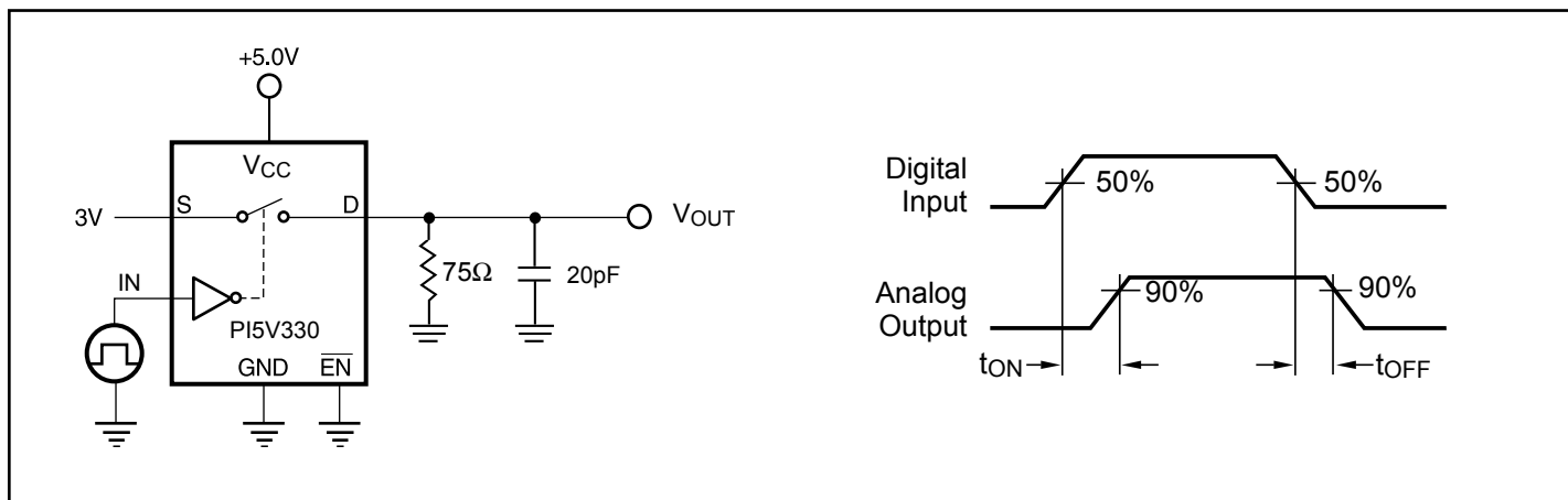
Figure 4. Switching Time
