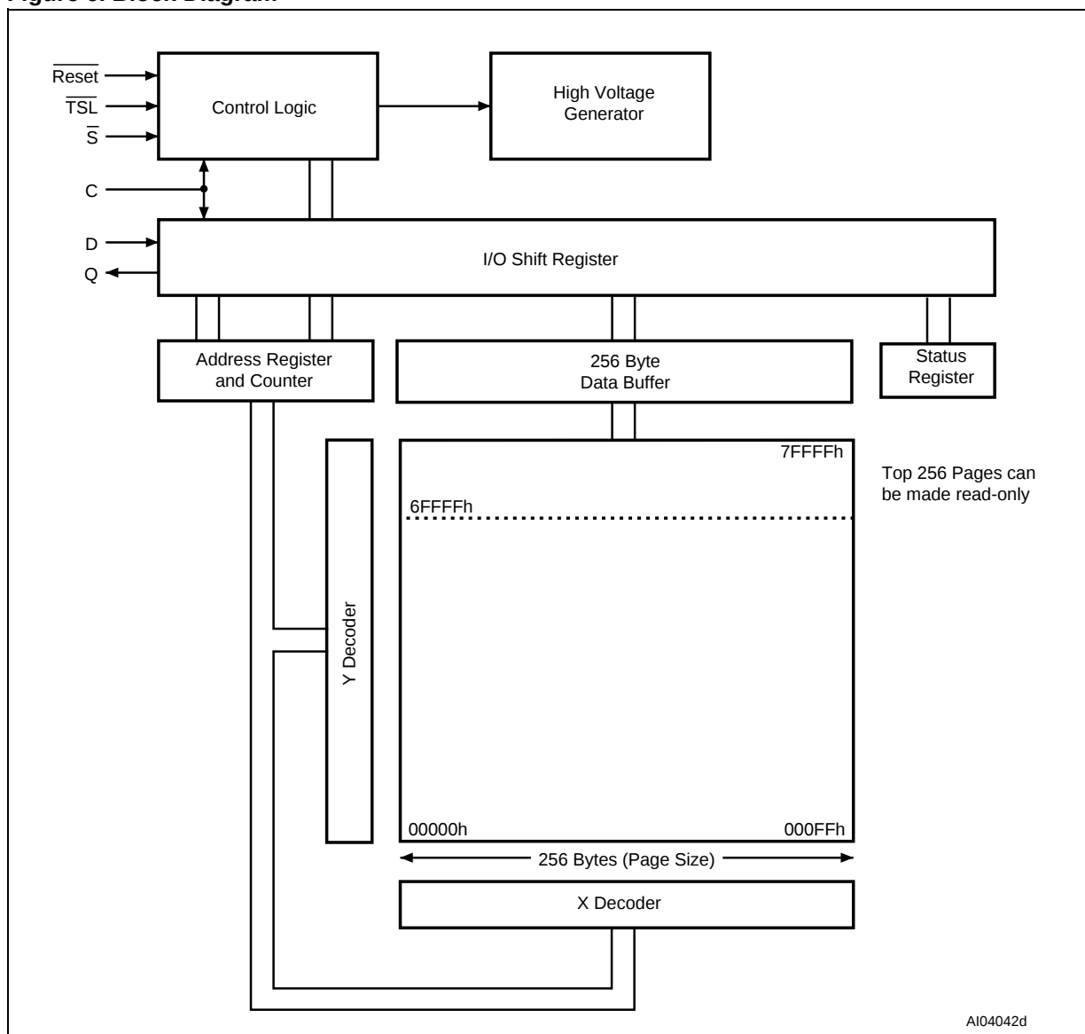
Figure 6. Block Diagram
