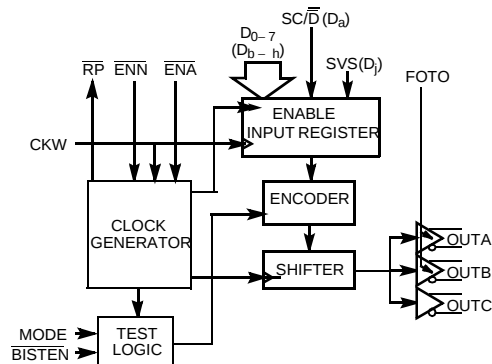
CY7B923 Transmitter
