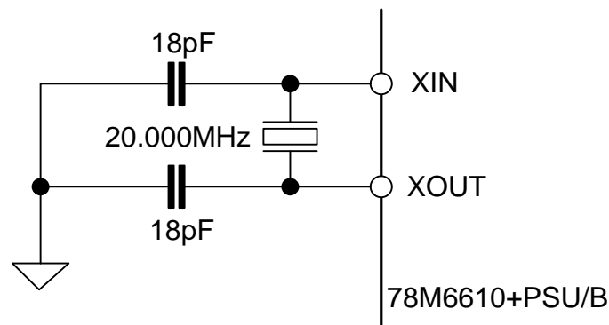
Figure 1-2: XTAL Connection
