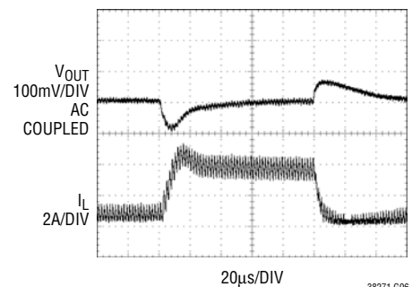
FIGURE 13 CIRCUIT V_{\text{OUT}} = 3.3\text{V}
