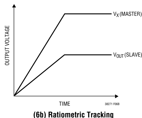
Figure 6. Two Different Modes of Output Voltage Tracking
