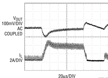
FIGURE 13 CIRCUIT V_{\text{OUT}} = 3.3\text{V}
