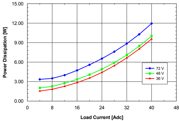
Fig. 1.0V.5: Power dissipation vs. load current and input voltage for QME48T40010 converter mounted horizontally with air flowing from pin 1 to pin 3 at a rate of 300 LFM (1.5 m/s) and T_a = 25^\circ\text{C} .
