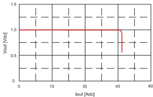
Fig. 1.0V.15: Output voltage vs. load current showing current limit point and converter shutdown point. Input voltage has almost no effect on current limit characteristic.
