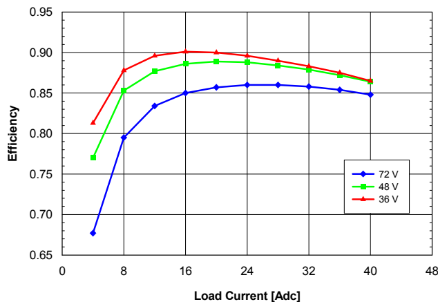
Fig. 1.8V.3: Efficiency vs. load current and input voltage for QME48T40018 converter mounted horizontally with air flowing from pin 1 to pin 3 at a rate of 300 LFM (1.5 m/s) and T_a = 25 °C.
