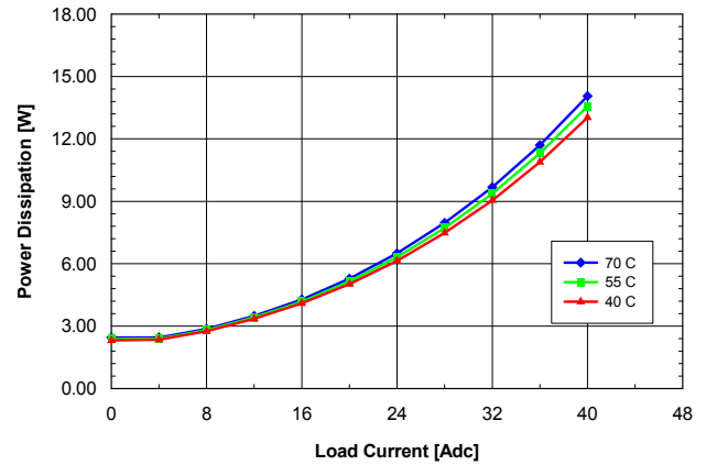
Fig. 2.5V.6: Power dissipation vs. load current and ambient temperature for QME48T40025 converter mounted horizontally with V_{in} = 48\text{ V} and air flowing from pin 1 to pin 3 at a rate of 200 LFM (1.0 m/s).
