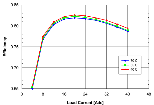
Fig. 1.0V.4: Efficiency vs. load current and ambient temperature for QME48T40010 converter mounted horizontally with V_{in} = 48\text{ V} and air flowing from pin 1 to pin 3 at a rate of 200 LFM (1.0 m/s).
