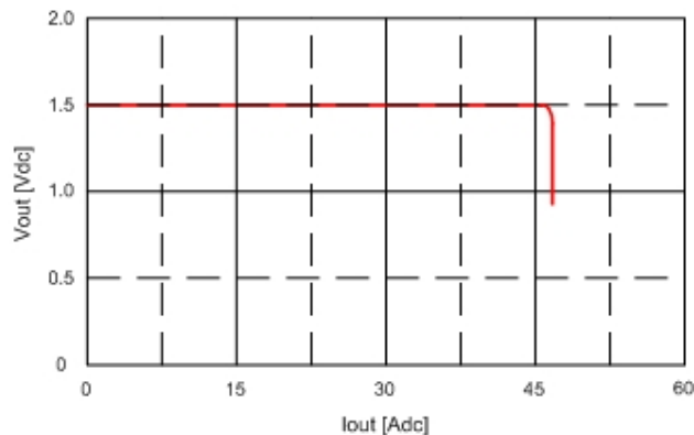
Fig. 1.5V.15: Output voltage vs. load current showing current limit point and converter shutdown point. Input voltage has almost no effect on current limit characteristic.
