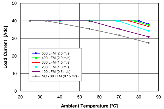
Fig. 1.0V.2: Available load current vs. ambient air temperature and airflow rates for QME48T40010 converter with G height pins mounted horizontally with air flowing from pin 1 to pin 3, MOSFET temperature \leq 120^{\circ}\text{C} , V_{in} = 48\text{ V} .
