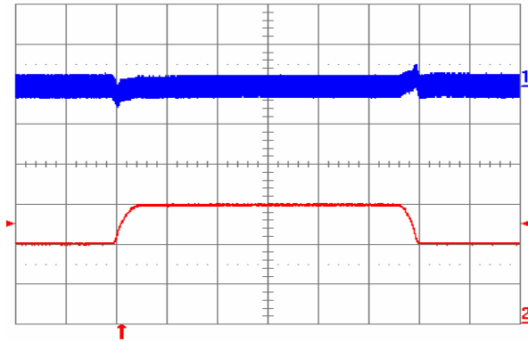
Fig. 3.3V.9: Output voltage response to load current step-change (20 A – 30 A – 20 A) at V_{in} = 48 V. Top trace: output voltage (100 mV/div.). Bottom trace: load current (10 A/div.). Current slew rate: 0.1 A/ \mu s. C_o = 1 \mu F ceramic. Time scale: 0.2 ms/div.
