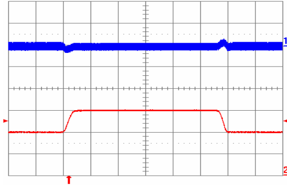
Fig. 1.5V.9: Output voltage response to load current step-change (20 A – 30 A – 20 A) at V_{in} = 48 V. Top trace: output voltage (100 mV/div.). Bottom trace: load current (10 A/div.). Current slew rate: 0.1 A/ \mu s. C_o = 1 \mu F ceramic. Time scale: 0.2 ms/div.
