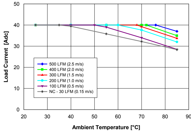
Fig. 1.8V.1: Available load current vs. ambient air temperature and airflow rates for QME48T40018 converter with G height pins mounted vertically with air flowing from pin 1 to pin 3, MOSFET temperature \leq 120 °C, V_{in} = 48 V.
