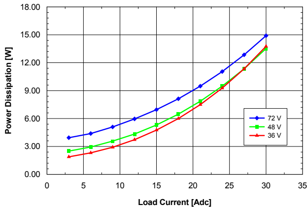
Fig. 3.3V.5: Power dissipation vs. load current and input voltage for QME48T40033 converter mounted horizontally with air flowing from pin 1 to pin 3 at a rate of 300 LFM (1.5 m/s) and T_a = 25^\circ\text{C} .
