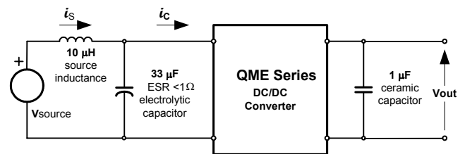
Fig. 1.2V.12: Test setup for measuring input reflected ripple currents, i_c and i_s .
