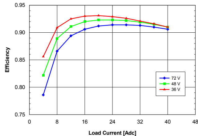
Fig. 3.3V.3: Efficiency vs. load current and input voltage for QME48T40033 converter mounted horizontally with air flowing from pin 1 to pin 3 at a rate of 300 LFM (1.5 m/s) and T_a = 25 °C.
