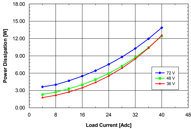
Fig. 2.5V.5: Power dissipation vs. load current and input voltage for QME48T40025 converter mounted horizontally with air flowing from pin 1 to pin 3 at a rate of 300 LFM (1.5 m/s) and T_a = 25^\circ\text{C} .
