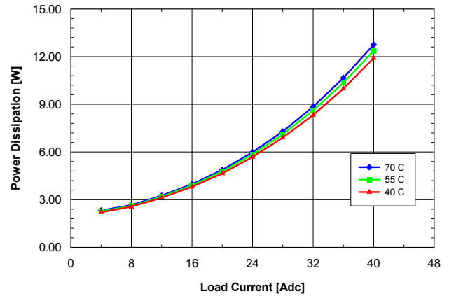
Fig. 1.8V.6: Power dissipation vs. load current and ambient temperature for QME48T40018 converter mounted horizontally with V_{in} = 48\text{ V} and air flowing from pin 1 to pin 3 at a rate of 200 LFM (1.0 m/s).
