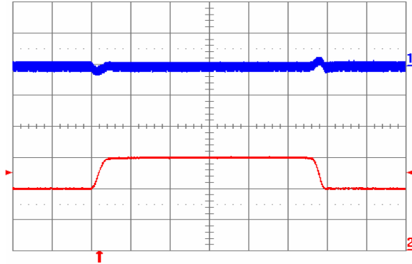
Fig. 1.2V.9: Output voltage response to load current step-change (20 A – 30 A – 20 A) at V_{in} = 48 V. Top trace: output voltage (100 mV/div.). Bottom trace: load current (10 A/div.). Current slew rate: 0.1 A/ \mu s. C_o = 1 \mu F ceramic. Time scale: 0.2 ms/div.
