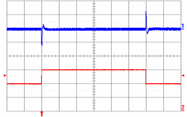
Fig. 1.8V.10: Output voltage response to load current step-change (20 A – 30 A – 20 A) at V_{in} = 48 V. Top trace: output voltage (100 mV/div.). Bottom trace: load current (10 A/div.). Current slew rate: 5 A/ \mu s. C_o = 470 \mu F POS + 1 \mu F ceramic. Time scale: 0.2 ms/div.
