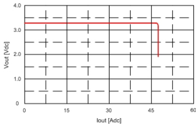
Fig. 3.3V.15: Output voltage vs. load current showing current limit point and converter shutdown point. Input voltage has almost no effect on current limit characteristic.
