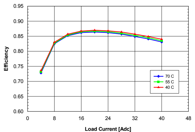
Fig. 1.5V.4: Efficiency vs. load current and ambient temperature for QME48T40015 converter mounted horizontally with V_{in} = 48\text{ V} and air flowing from pin 1 to pin 3 at a rate of 200 LFM (1.0 m/s).
