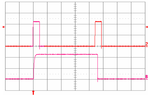
Fig. 1.2V.16: Load current (top trace, 20 A/div., 50 ms/div.) into a 10 m\Omega short circuit during restart, at V_{in} = 48 V. Bottom trace (20 A/div., 5 ms/div.) is an expansion of the on-time portion of the top trace.
