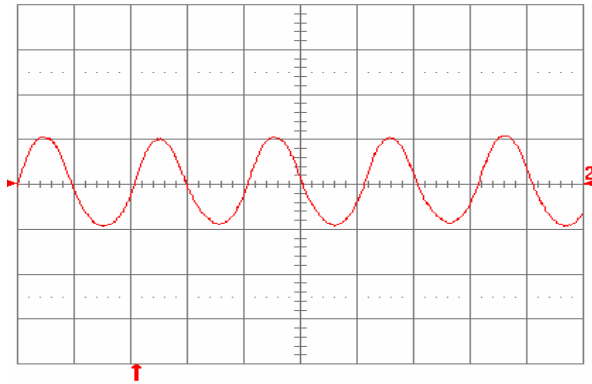
Fig. 3.3V.13: Input reflected ripple current, i_c (100 mA/div.), measured at input terminals at full rated load current and V_{in} = 48 V. Refer to Fig. 3.3V.12 for test setup. Time scale: 1 \mu s/div.
