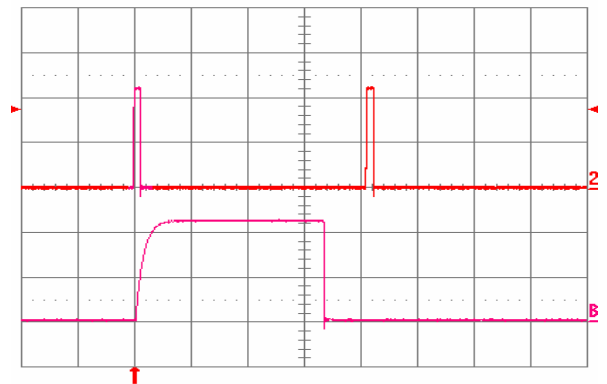
Fig. 3.3V.16: Load current (top trace, 20 A/div., 50 ms/div.) into a 10 m \Omega short circuit during restart, at V_{in} = 48 V. Bottom trace (20 A/div., 2 ms/div.) is an expansion of the on-time portion of the top trace.
