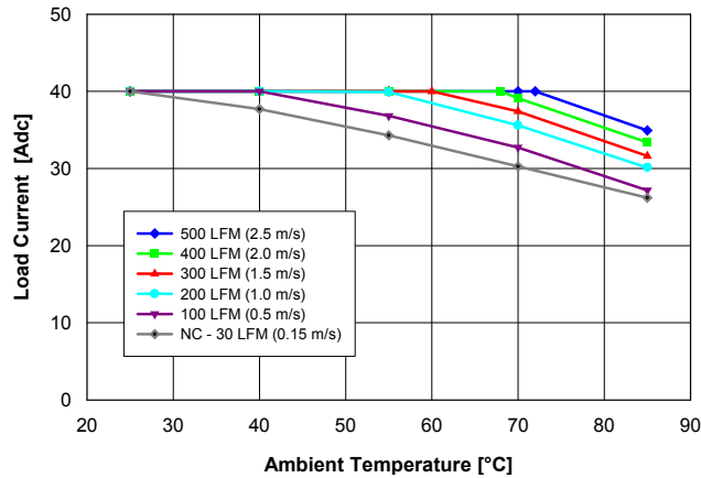
Fig. 2.5V.1: Available load current vs. ambient air temperature and airflow rates for QME48T40025 converter with G height pins mounted vertically with air flowing from pin 1 to pin 3, MOSFET temperature \leq 120^{\circ}\text{C} , V_{in} = 48\text{ V} .
