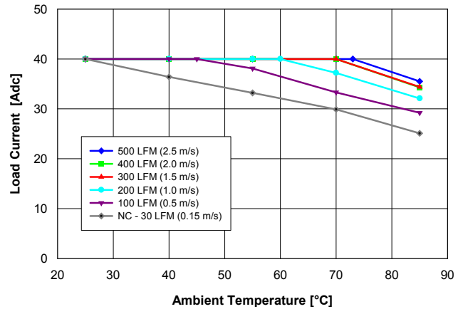
Fig. 1.8V.2: Available load current vs. ambient air temperature and airflow rates for QME48T40018 converter with G height pins mounted horizontally with air flowing from pin 1 to pin 3, MOSFET temperature \leq 120 °C, V_{in} = 48 V.
