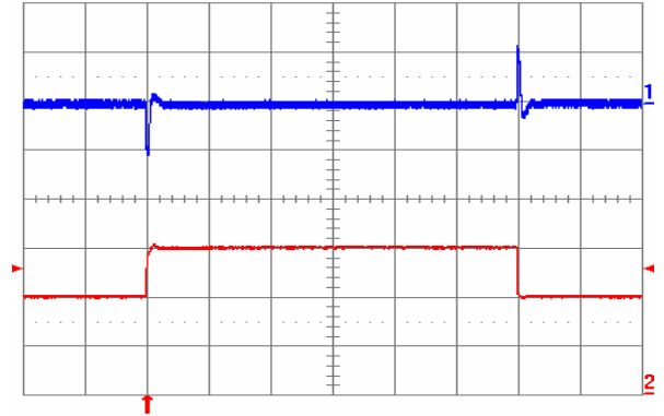
Fig. 1.2V.10: Output voltage response to load current step-change (20 A – 30 A – 20 A) at V_{in} = 48 V. Top trace: output voltage (100 mV/div.). Bottom trace: load current (10 A/div.). Current slew rate: 5 A/ \mu s. C_o = 470 \mu F POS + 1 \mu F ceramic. Time scale: 0.2 ms/div.
