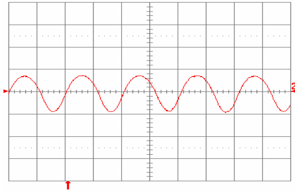
Fig. 1.8V.13: Input reflected ripple current, i_c (100 mA/div.), measured at input terminals at full rated load current and V_{in} = 48 V. Refer to Fig. 1.8V.12 for test setup. Time scale: 1 \mu s/div.
