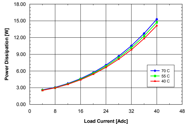
Fig. 3.3V.6: Power dissipation vs. load current and ambient temperature for QME48T40033 converter mounted horizontally with V_{in} = 48\text{ V} and air flowing from pin 1 to pin 3 at a rate of 200 LFM (1.0 m/s).
