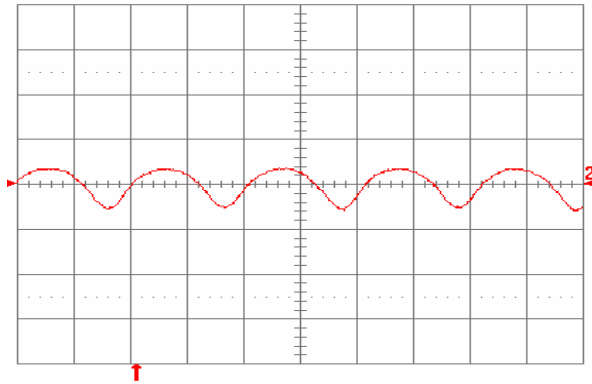
Fig. 1.0V.13: Input reflected ripple current, i_c (100 mA/div.), measured at input terminals at full rated load current and V_{in} = 48 V. Refer to Fig. 1.0V.12 for test setup. Time scale: 1 \mu s/div.
