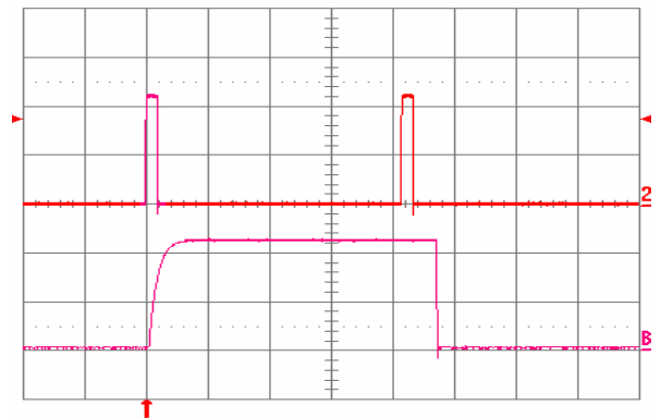
Fig. 2.5V.16: Load current (top trace, 20 A/div., 50 ms/div.) into a 10 m\Omega short circuit during restart, at V_{in} = 48 V. Bottom trace (20 A/div., 2 ms/div.) is an expansion of the on-time portion of the top trace.
