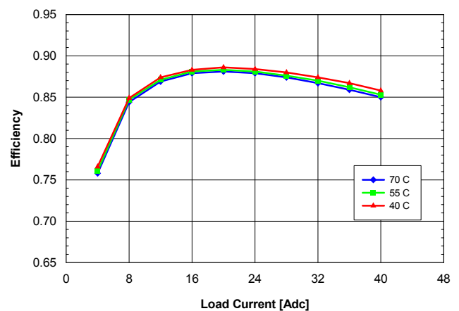
Fig. 1.8V.4: Efficiency vs. load current and ambient temperature for QME48T40018 converter mounted horizontally with V_{in} = 48 V and air flowing from pin 1 to pin 3 at a rate of 200 LFM (1.0 m/s).
