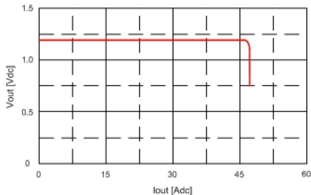
Fig. 1.2V.15: Output voltage vs. load current showing current limit point and converter shutdown point. Input voltage has almost no effect on current limit characteristic.
