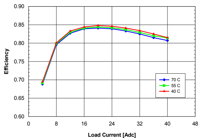
Fig. 1.2V.4: Efficiency vs. load current and ambient temperature for QME48T40012 converter mounted horizontally with V_{in} = 48 V and air flowing from pin 1 to pin 3 at a rate of 200 LFM (1.0 m/s).
