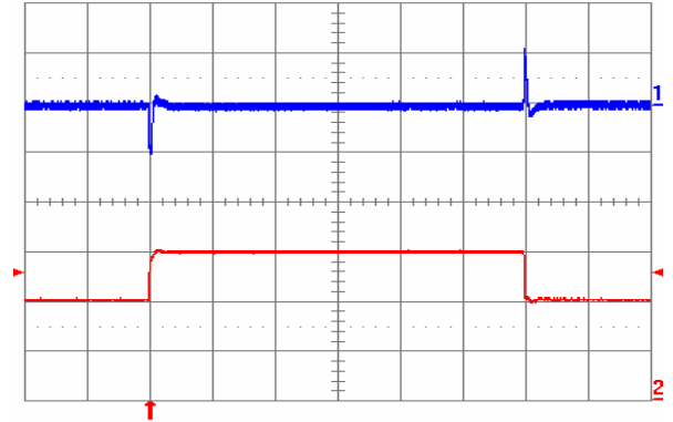
Fig. 1.0V.10: Output voltage response to load current step-change (20 A – 30 A – 20 A) at V_{in} = 48 V. Top trace: output voltage (100 mV/div.). Bottom trace: load current (10 A/div.). Current slew rate: 5 A/ \mu s. C_o = 470 \mu F POS + 1 \mu F ceramic. Time scale: 0.2 ms/div.
