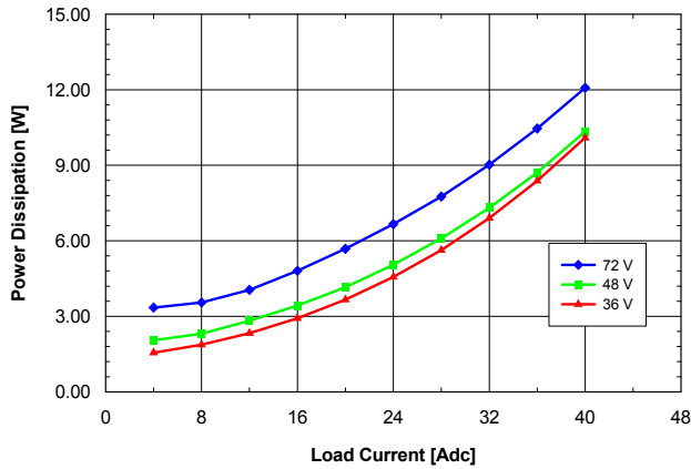
Fig. 1.2V.5: Power dissipation vs. load current and input voltage for QME48T40012 converter mounted horizontally with air flowing from pin 1 to pin 3 at a rate of 300 LFM (1.5 m/s) and T_a = 25^\circ\text{C} .
