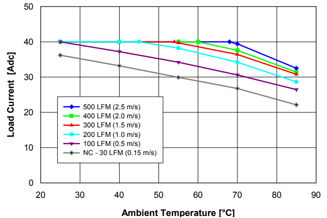
Fig. 3.3V.2: Available load current vs. ambient air temperature and airflow rates for QME48T40033 converter with G height pins mounted horizontally with air flowing from pin 1 to pin 3, MOSFET temperature \leq 120 °C, V_{in} = 48 V.
