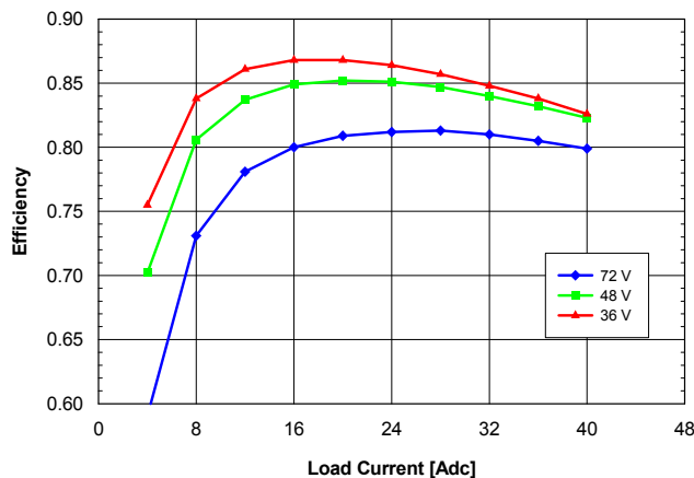
Fig. 1.2V.3: Efficiency vs. load current and input voltage for QME48T40012 converter mounted horizontally with air flowing from pin 1 to pin 3 at a rate of 300 LFM (1.5 m/s) and T_a = 25 °C.
