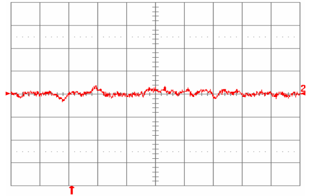
Fig. 1.0V.14: Input reflected ripple current, i_s (10 mA/div.), measured through 10 \mu H at the source at full rated load current and V_{in} = 48 V. Refer to Fig. 1.0V.12 for test setup. Time scale: 1 \mu s/div.
