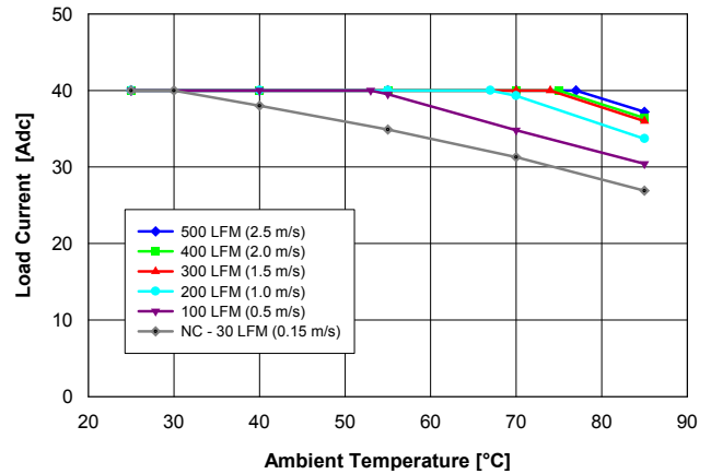
Fig. 1.2V.2: Available load current vs. ambient air temperature and airflow rates for QME48T40012 converter with G height pins mounted horizontally with air flowing from pin 1 to pin 3, MOSFET temperature \leq 120 °C, V_{in} = 48 V.
