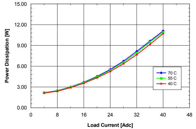
Fig. 1.2V.6: Power dissipation vs. load current and ambient temperature for QME48T40012 converter mounted horizontally with V_{in} = 48\text{ V} and air flowing from pin 1 to pin 3 at a rate of 200 LFM (1.0 m/s).
