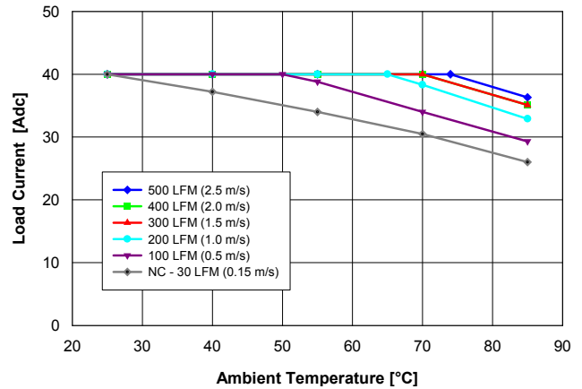
Fig. 1.5V.2: Available load current vs. ambient air temperature and airflow rates for QME48T40015 converter with G height pins mounted horizontally with air flowing from pin 1 to pin 3, MOSFET temperature \leq 120^{\circ}\text{C} , V_{in} = 48\text{ V} .
