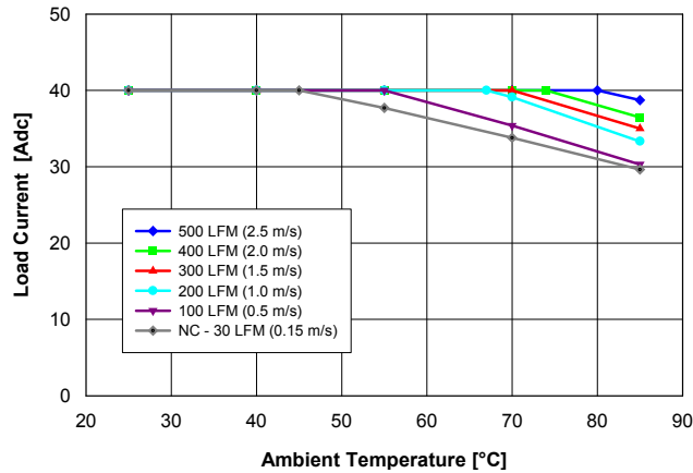
Fig. 1.2V.1: Available load current vs. ambient air temperature and airflow rates for QME48T40012 converter with G height pins mounted vertically with air flowing from pin 1 to pin 3, MOSFET temperature \leq 120 °C, V_{in} = 48 V.
