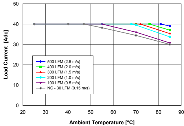
Fig. 1.0V.1: Available load current vs. ambient air temperature and airflow rates for QME48T40010 converter with G height pins mounted vertically with air flowing from pin 1 to pin 3, MOSFET temperature \leq 120^{\circ}\text{C} , V_{in} = 48\text{ V} .
