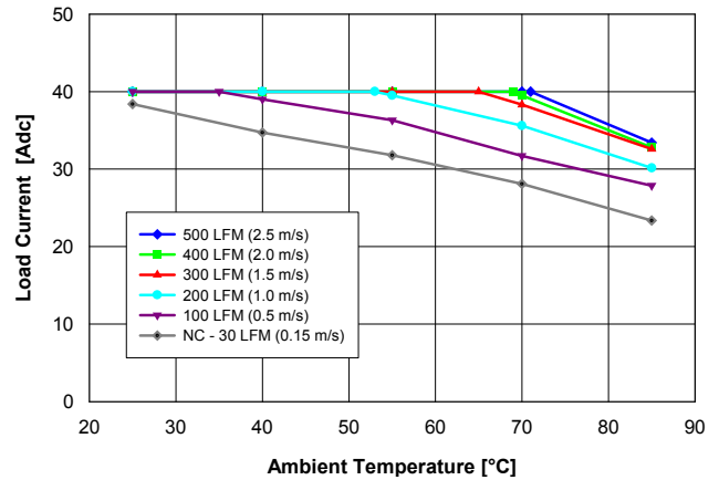
Fig. 2.5V.2: Available load current vs. ambient air temperature and airflow rates for QME48T40025 converter with G height pins mounted horizontally with air flowing from pin 1 to pin 3, MOSFET temperature \leq 120^{\circ}\text{C} , V_{in} = 48\text{ V} .
