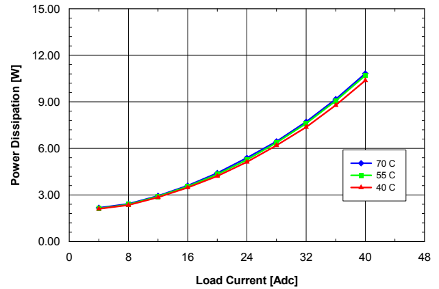
Fig. 1.0V.6: Power dissipation vs. load current and ambient temperature for QME48T40010 converter mounted horizontally with V_{in} = 48\text{ V} and air flowing from pin 1 to pin 3 at a rate of 200 LFM (1.0 m/s).
