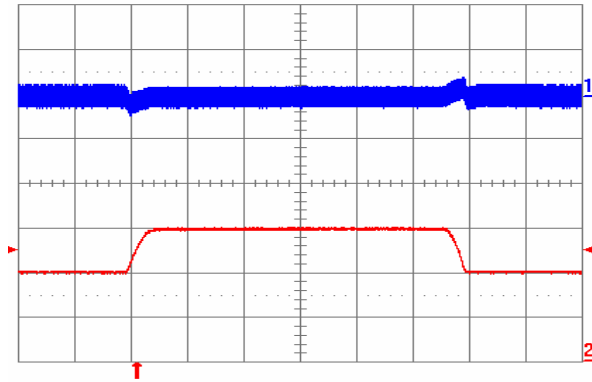
Fig. 2.5V.9: Output voltage response to load current step-change (20 A – 30 A – 20 A) at V_{in} = 48 V. Top trace: output voltage (100 mV/div.). Bottom trace: load current (10 A/div.). Current slew rate: 0.1 A/ \mu s. C_o = 1 \mu F ceramic. Time scale: 0.2 ms/div.
