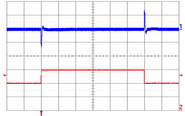
Fig. 2.5V.10: Output voltage response to load current step-change (20 A – 30 A – 20 A) at V_{in} = 48 V. Top trace: output voltage (100 mV/div.). Bottom trace: load current (10 A/div.). Current slew rate: 5A/ \mu s. C_o = 470 \mu F POS + 1 \mu F ceramic. Time scale: 0.2 ms/div.
