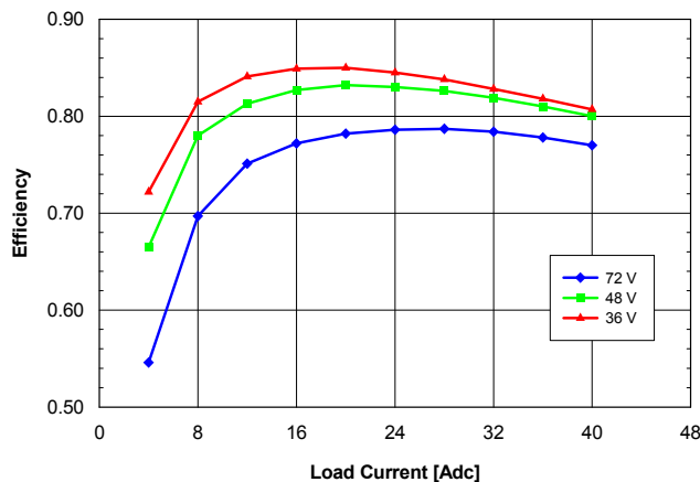
Fig. 1.0V.3: Efficiency vs. load current and input voltage for QME48T40010 converter mounted horizontally with air flowing from pin 1 to pin 3 at a rate of 300 LFM (1.5 m/s) and T_a = 25^{\circ}\text{C} .
