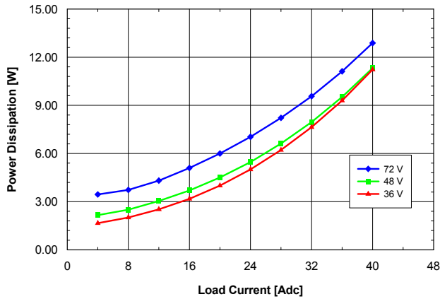
Fig. 1.8V.5: Power dissipation vs. load current and input voltage for QME48T40018 converter mounted horizontally with air flowing from pin 1 to pin 3 at a rate of 300 LFM (1.5 m/s) and T_a = 25^\circ\text{C} .
