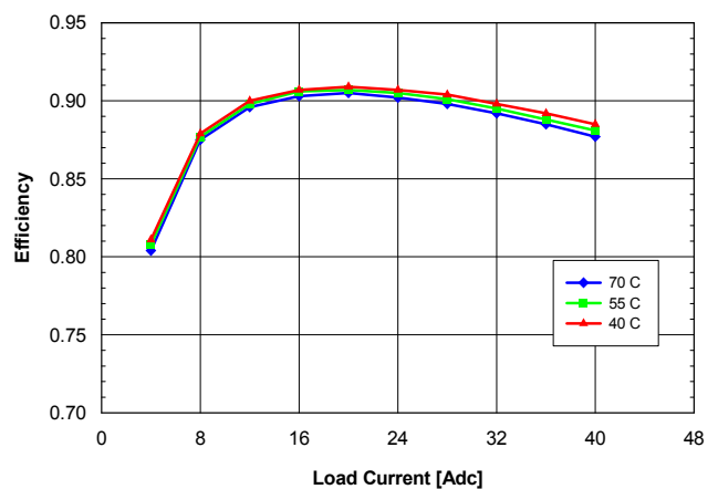
Fig. 2.5V.4: Efficiency vs. load current and ambient temperature for QME48T40025 converter mounted horizontally with V_{in} = 48\text{ V} and air flowing from pin 1 to pin 3 at a rate of 200 LFM (1.0 m/s).
