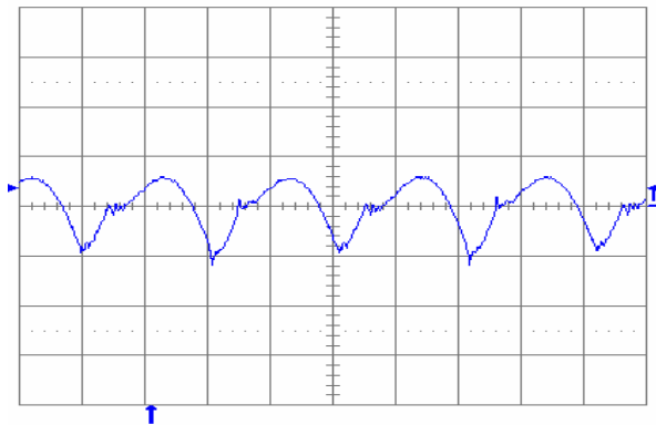
Fig. 1.0V.11: Output voltage ripple (20 mV/div.) at full rated load current into a resistive load with C_o = 10 \mu F tantalum + 1 \mu F ceramic and V_{in} = 48 V. Time scale: 1 \mu s/div.
