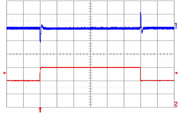
Fig. 1.5V.10: Output voltage response to load current step-change (20 A – 30 A – 20 A) at V_{in} = 48 V. Top trace: output voltage (100 mV/div.). Bottom trace: load current (10 A/div.). Current slew rate: 5A/ \mu s. C_o = 470 \mu F POS + 1 \mu F ceramic. Time scale: 0.2 ms/div.
