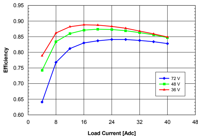
Fig. 1.5V.3: Efficiency vs. load current and input voltage for QME48T40015 converter mounted horizontally with air flowing from pin 1 to pin 3 at a rate of 300 LFM (1.5 m/s) and T_a = 25^{\circ}\text{C} .
