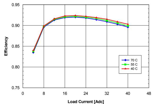
Fig. 3.3V.4: Efficiency vs. load current and ambient temperature for QME48T40033 converter mounted horizontally with V_{in} = 48 V and air flowing from pin 1 to pin 3 at a rate of 200 LFM (1.0 m/s).
