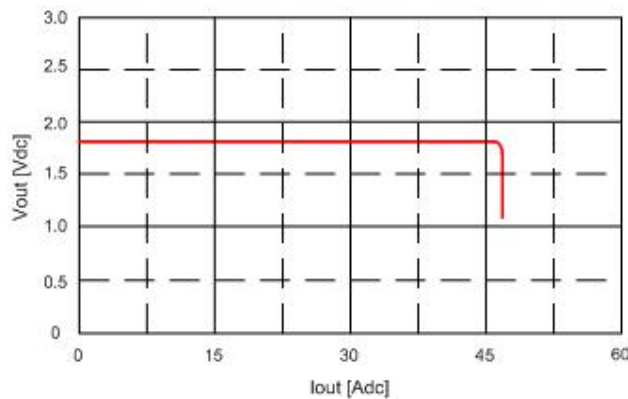
Fig. 1.8V.15: Output voltage vs. load current showing current limit point and converter shutdown point. Input voltage has almost no effect on current limit characteristic.
