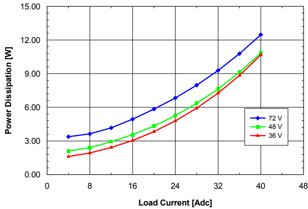
Fig. 1.5V.5: Power dissipation vs. load current and input voltage for QME48T40015 converter mounted horizontally with air flowing from pin 1 to pin 3 at a rate of 300 LFM (1.5 m/s) and T_a = 25^\circ\text{C} .
