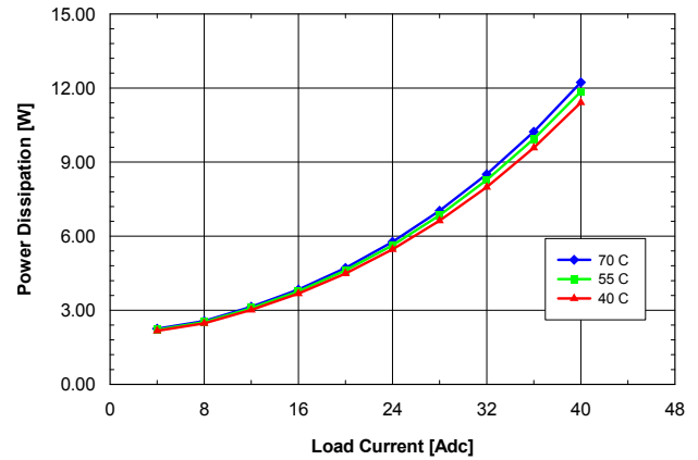
Fig. 1.5V.6: Power dissipation vs. load current and ambient temperature for QME48T40015 converter mounted horizontally with V_{in} = 48\text{ V} and air flowing from pin 1 to pin 3 at a rate of 200 LFM (1.0 m/s).
