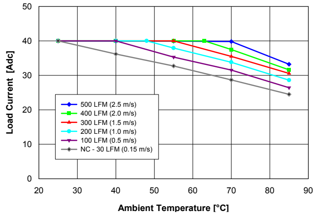
Fig. 3.3V.1: Available load current vs. ambient air temperature and airflow rates for QME48T40033 converter with G height pins mounted vertically with air flowing from pin 1 to pin 3, MOSFET temperature \leq 120 °C, V_{in} = 48 V.
