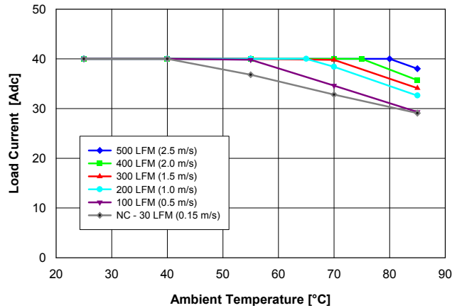
Fig. 1.5V.1: Available load current vs. ambient air temperature and airflow rates for QME48T40015 converter with G height pins mounted vertically with air flowing from pin 1 to pin 3, MOSFET temperature \leq 120^{\circ}\text{C} , V_{in} = 48\text{ V} .
