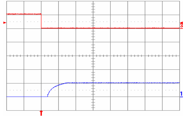
Fig. 1.0V.8: Turn-on transient at full rated load current (resistive) plus 10,000 \mu\text{F} at V_{in} = 48\text{ V} , triggered via ON/OFF pin. Top trace: ON/OFF signal (5 V/div.). Bottom trace: output voltage (1 V/div.). Time scale: 2 ms/div.
