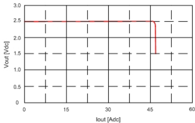
Fig. 2.5V.15: Output voltage vs. load current showing current limit point and converter shutdown point. Input voltage has almost no effect on current limit characteristic.
