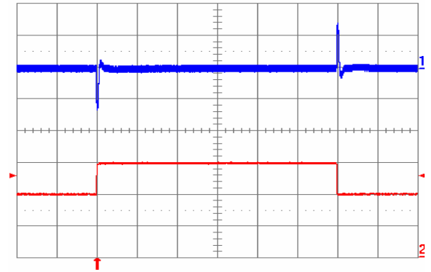
Fig. 3.3V.10: Output voltage response to load current step-change (20 A – 30 A – 20 A) at V_{in} = 48 V. Top trace: output voltage (100 mV/div.). Bottom trace: load current (10 A/div.). Current slew rate: 5 A/ \mu s. C_o = 470 \mu F POS + 1 \mu F ceramic. Time scale: 0.2 ms/div.
