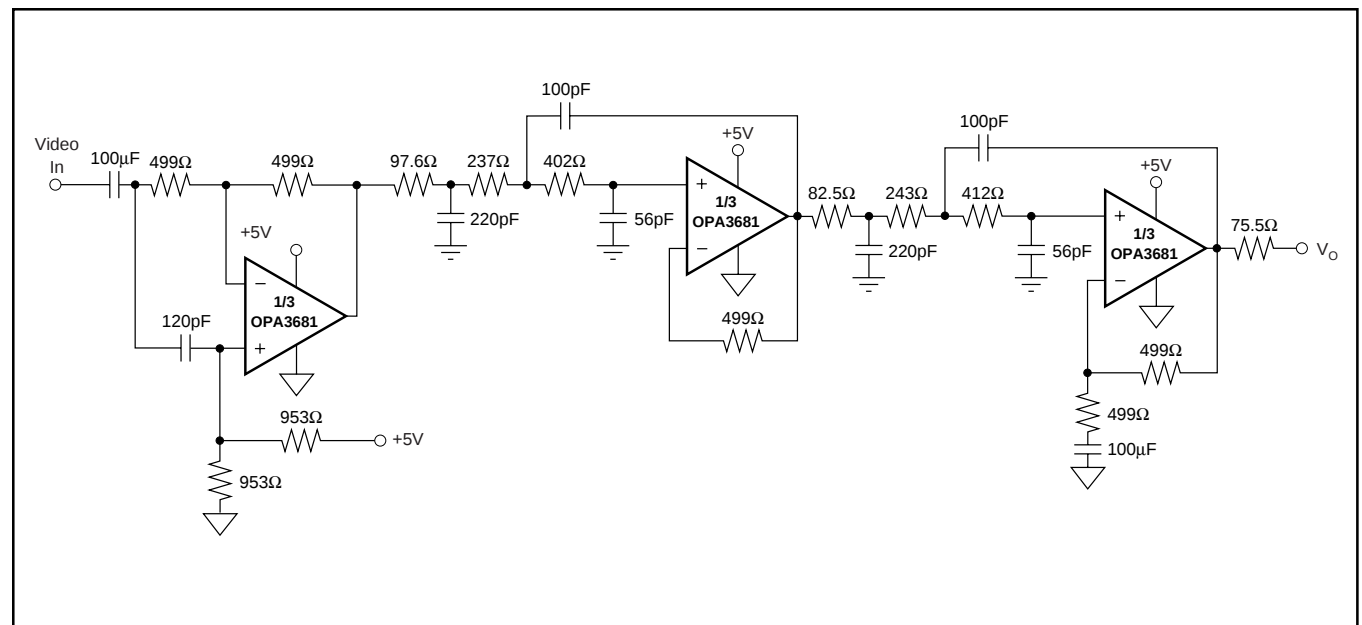
FIGURE 5. Filter Schematic.
