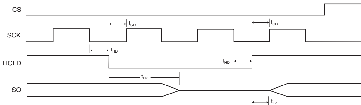
Figure 10. HOLD Timing
