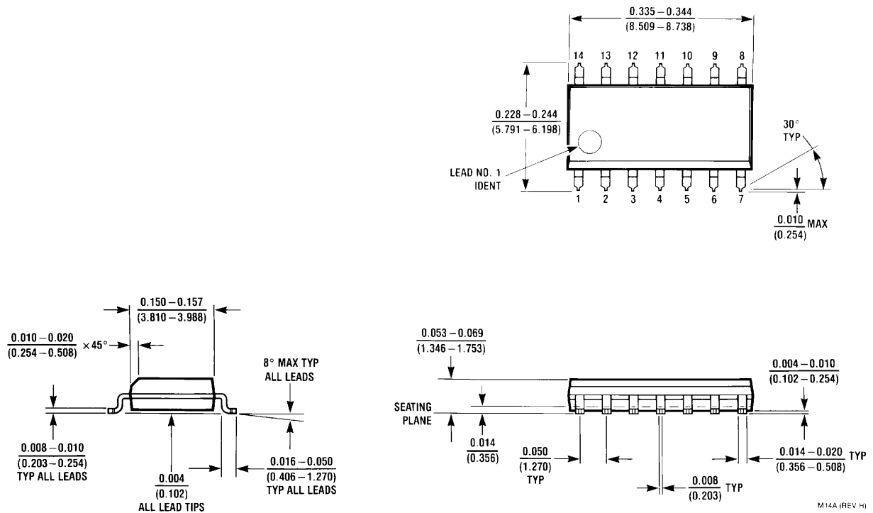
14-Lead (0.300" Wide) Molded Small Outline Package, JEDEC NS Package Number M14A
