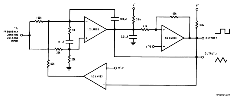
Two-Decade High Frequency VCO
