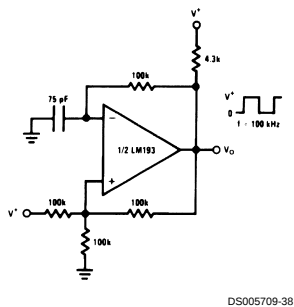
Squarewave Oscillator
