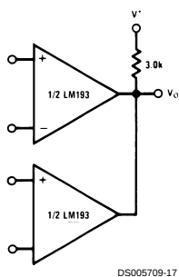
ORing the Outputs
