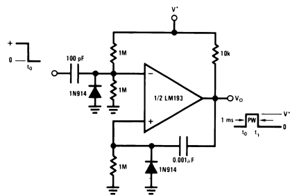
One-Shot Multivibrator
