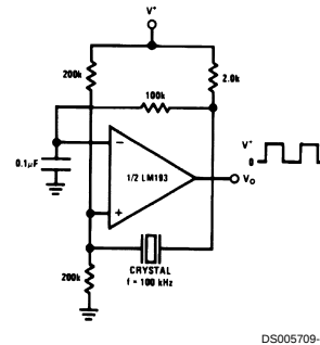
Crystal Controlled Oscillator
