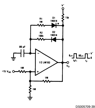
Pulse Generator
