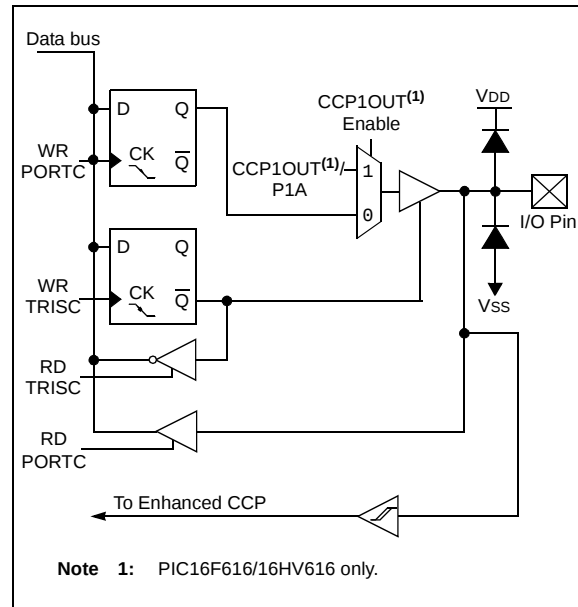
FIGURE 4-9: BLOCK DIAGRAM OF RC5 PIN
