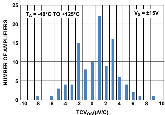
FIGURE 4. T_C V_{OS} DISTRIBUTION, -40^\circ C to +125^\circ C
