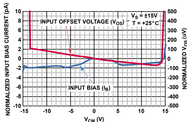
FIGURE 44. INPUT OFFSET VOLTAGE AND BIAS CURRENT vs COMMON MODE INPUT VOLTAGE
