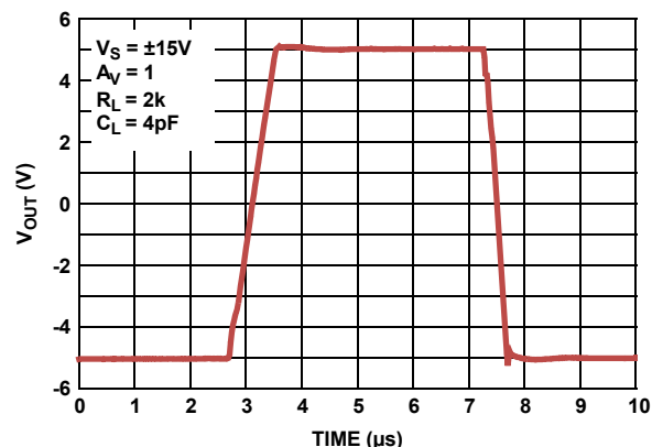
FIGURE 38. LARGE SIGNAL UNITY GAIN TRANSIENT RESPONSE
