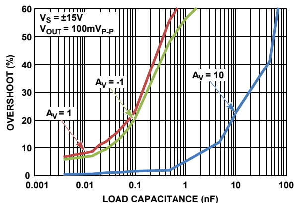
FIGURE 24. SMALL SIGNAL OVERSHOOT vs LOAD CAPACITANCE ( C_L )
