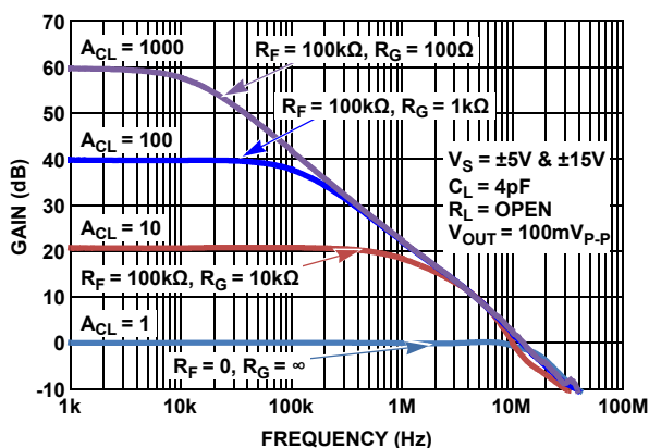
FIGURE 26. CLOSED LOOP GAIN vs FREQUENCY
