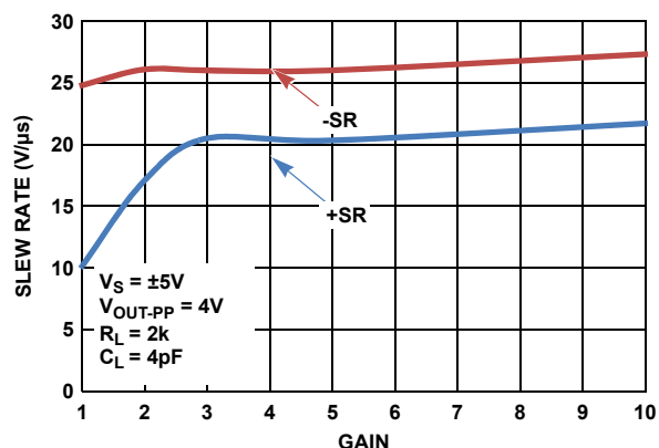
FIGURE 35. SLEW RATE vs NON-INVERTING CLOSED LOOP GAIN, V_S = \pm 5V
