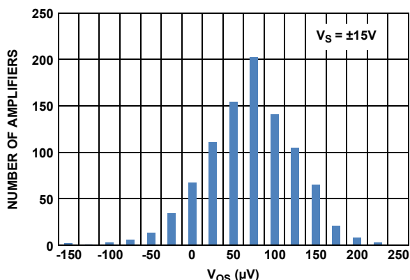
FIGURE 3. INPUT OFFSET VOLTAGE ( V_{OS} ) DISTRIBUTION
