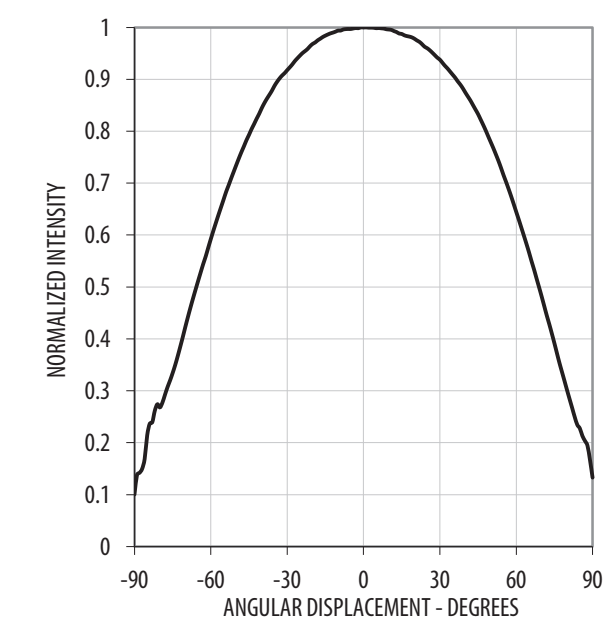
Figure 5: Radiation Pattern
