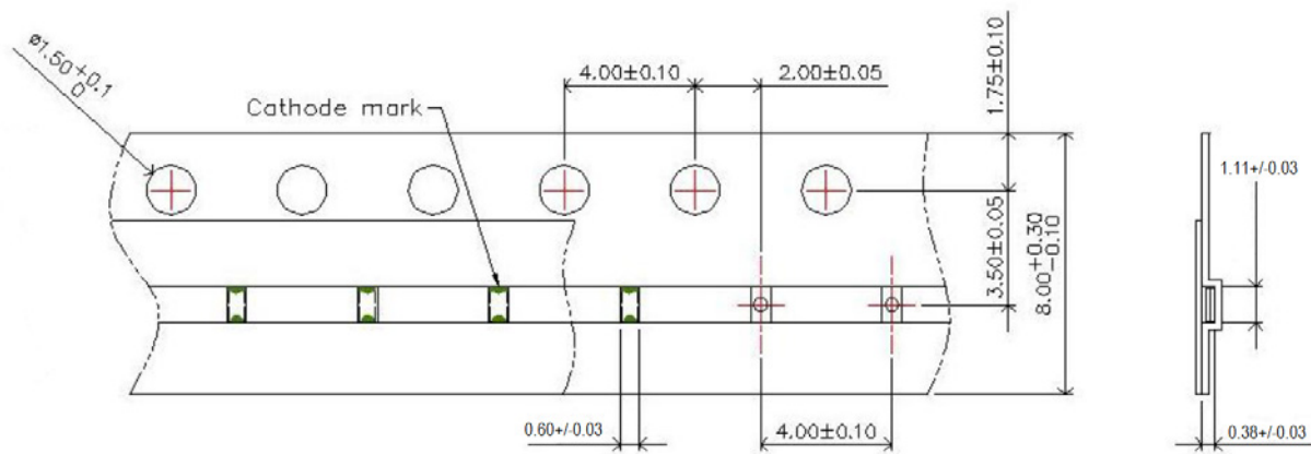
Figure 14: Carrier Tape Dimensions (Units: mm)
