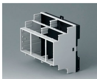
B6504121 RAILTEC B, 6 modules, Vers. VI PC (UL 94 V-0) light gray RAL 7035 4.13"x3.54"x2.28"
