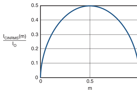
Figure 2. I_{CIN} vs. Voltage Conversion Ratio
