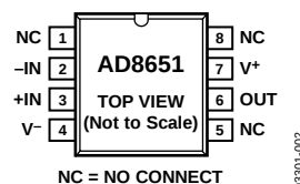
Figure 3. 8-Lead SOIC_N (R-8)
