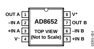
Figure 4. 8-Lead SOIC_N (R-8)
