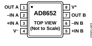
Figure 2. 8-Lead MSOP (RM-8)
