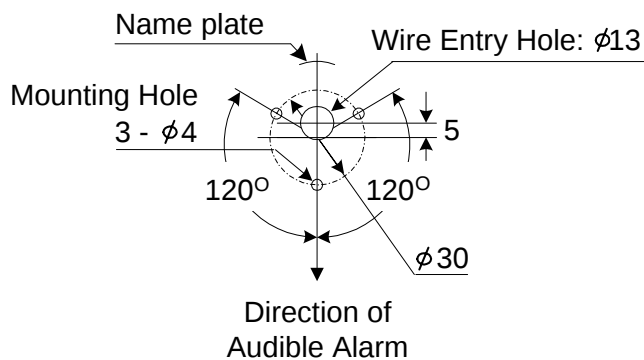
Mounting Dimensions
