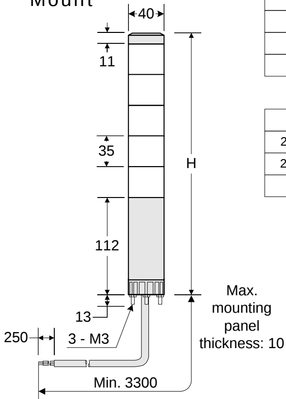
Direct Mount
