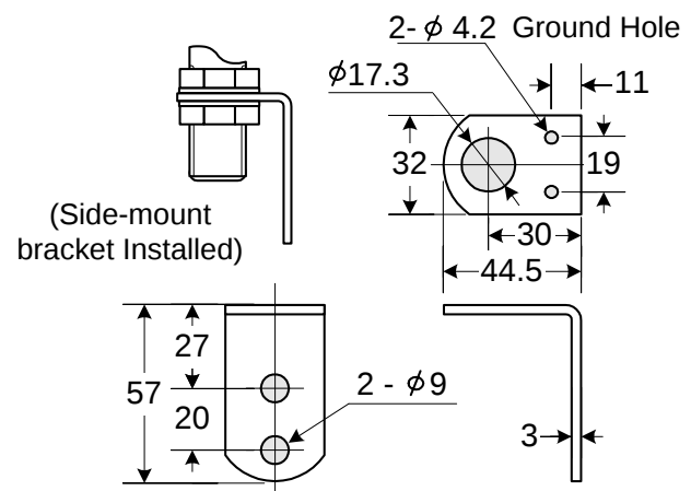
Side-mount Bracket (Supplied)
