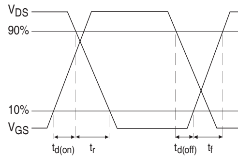
Fig 15b. Switching Time Waveforms www.irf.com
