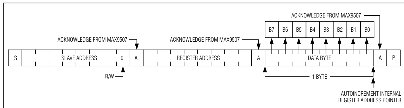
Figure 8. Writing a Byte of Data to the MAX9507
