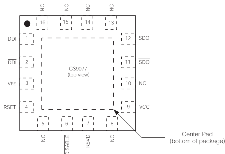
Figure 1-1: 16-Pin QFN
