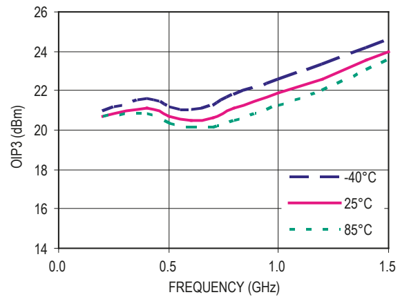
Figure 22. OIP3 vs Frequency ( V_d = 3V , I_{ds} = 15mA )
